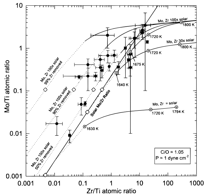
FIG. 11.—Measured Mo/Ti and Zr/Ti atomic ratios in carbides from circumstellar graphite (data from Table 1) compared with calculated condensation tracks for ideal solid solutions ( curves ). The curves are labeled “solar,” “30 × solar” and “100 × solar” to indicate overall Mo and Zr abundances used in the calculations. Curves for some percentage removal of Zr (50%, 90%, 99%) are also shown for the 100 × solar case. Condensation starts out with the formation of Zr-rich grains ( solid curves ). The switch from solid to dotted curves occurs where \sim 10\% of total Ti is condensed. Dotted circles are temperature markers. The diagonal straight line is the locus of solar Mo/Zr ratios. The open diamonds on this line indicate (starting from lower left), solar, 30 times solar, and 100 times solar (Mo, Zr)/Ti ratios when all three elements are completely condensed. The open diamonds on the dotted curves indicate the final grain compositions for cases of Zr removal.
