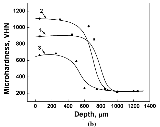
Fig. 3—Variation of microhardness with depth from the surface of laser-surface-nitrided Ti-6Al-4V showing the effect of (a) applied power lased at a nitrogen gas flow rate of 10 L/min and power of 600 W (plot 1), 700 W (plot 2), and (3) 800 W (plot 3), and (b) nitrogen gas flow rate lased at an applied power of 700 W and gas flow rate of 5 L/min (plot 1), 10 L/min (plot 2), and 20 L/min (plot 3).
