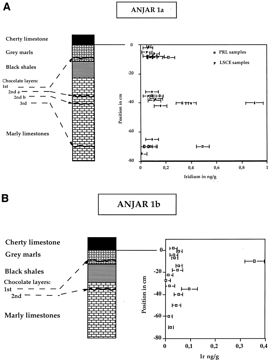
Fig. 2. Iridium measurements (in \text{ng g}^{-1} ) in three sections of intertrapean sediments IT3 at three nearby locations (all within the site shown as a star in Fig. 1). In each case a simplified geological section with rock types and sedimentary observations, and an iridium profile are shown. (A) Anjar 1a, (B) Anjar 1b and (C) Anjar 2. The samples measured in the Physical Research Laboratory in Ahmedabad, India, are marked PRL; those measured in the Laboratoire des Sciences du Climat et de l'Environnement in Gif-sur-Yvette, France, are marked SCE.
