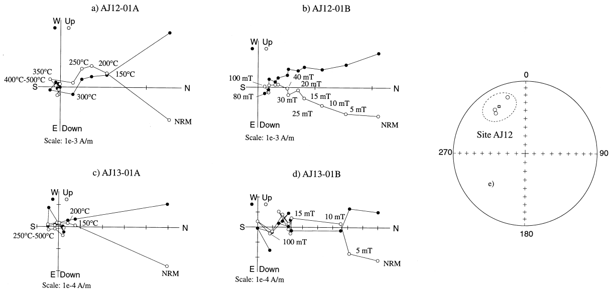
Fig. 6. Examples of AF and TH demagnetisation diagrams for samples from intertrappean sediments below (AJ12) and above (AJ13) the iridium levels. See caption of Fig. 4 for specifications. An equal area projection for the three samples for which a clear magnetic component could be isolated is shown at the right of the figure.
