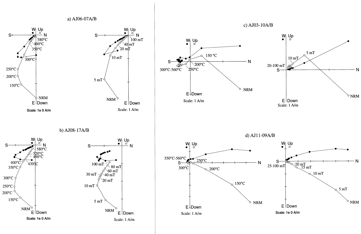
Fig. 4. Examples of AF and TH demagnetisation diagrams for samples from flows F9 (a), F6 (b), F3 (c) and F1 (d). Temperatures in °C and fields in mT. Solid symbols are in the horizontal plane and open symbols in the NS vertical plane. Intensities for space between tick marks on axes are given at the bottom of each diagram in A m -1 .
