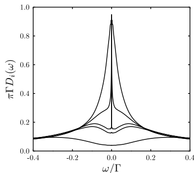
FIG. 3: Transmission \pi\Gamma D_i(\omega) vs \omega/\Gamma , for \tilde{U} = 7 and (top to bottom) \tilde{U}' = 7, 7.03, 7.044 (SC) and 7.048, 7.1 (CO).
