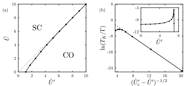
FIG. 1: (a) Phase diagram in (\tilde{U}', \tilde{U}) -plane; the SU(4) line U' = U is also shown (dotted). (b) For \tilde{U} = 7 in the SC phase, \ln(T_K/\Gamma) vs [\tilde{U}'_c - \tilde{U}']^{-1/2} close to the transition, showing the exponential vanishing of T_K . Inset: \ln(T_K/\Gamma) vs \tilde{U}' .
