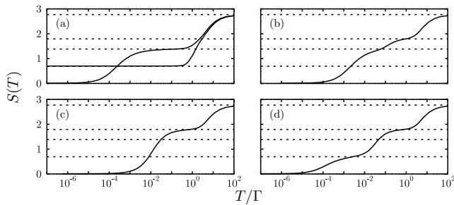
FIG. 2: S(T) vs T/\Gamma for \tilde{U} = 7 ( \tilde{U}'_c \simeq 7.046 ). (a) \tilde{U}' = 6 (SC, ‘uncoupled spin-Kondo’) and 8 (CO); (b) \tilde{U}' = 6.9 (crossover to SU(4) ); (c) \tilde{U}' = 7 ( SU(4) ); (d) \tilde{U}' = 7.03 (charge-Kondo). Dotted lines show \ln 16 , \ln 6 , \ln 4 and \ln 2 , associated with the FO, LM^{SU(4)} , LM^{SU(2)} and CO fixed points respectively.
