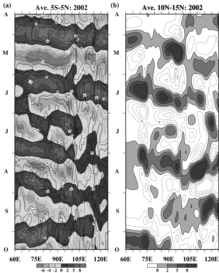
Figure 8. (a) Time-longitude variation of 20–80-day filtered TRMM 3B42 rainfall and filtered SST (contour) anomalies averaged over the equator (5°S–5°N) and (b) filtered observed rainfall averaged over the off-equatorial region (10°N–15°N).
