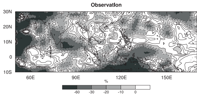
Figure 1. 2002 JJAS mean rainfall departure as percentage of climatological JJAS mean based on TRMM 3B42 rainfall.
