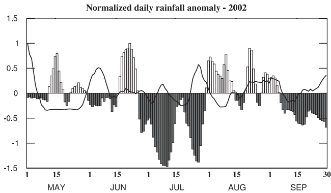
Figure 3. Normalized daily rainfall anomalies during 2002 summer season based on TRMM 3B42 rainfall data. The bars represent average over the central Indian region (MCZ) and the line represents average over the equatorial Indian Ocean (EQIO).
