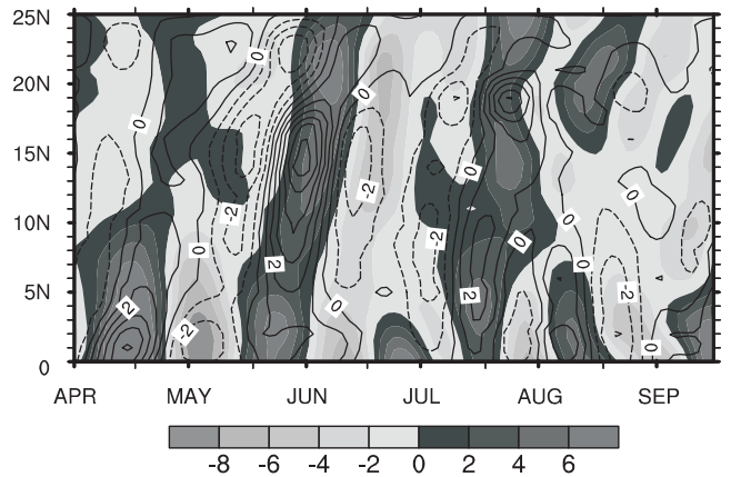
Figure 7. Time–latitude variation of 20–80-day filtered TRMM 3B42 rainfall anomalies averaged over 75°E–85°E (shaded) and filtered TMI surface zonal wind speed anomalies (contours) averaged over western Indian Ocean (50°E–80°E).
