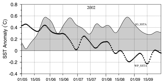
Figure 5. SST anomalies averaged over equatorial Indian Ocean (denoted as IO_SSTA) and western Pacific (denoted as WP_SSTA) during 2002.
