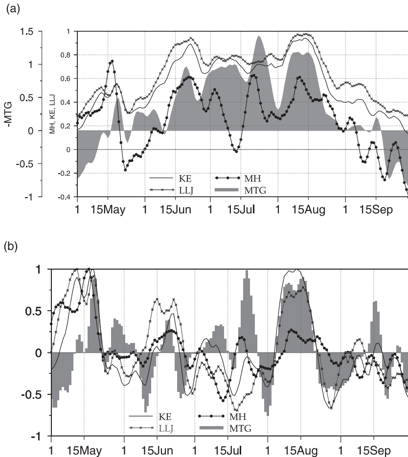
Figure 6. Daily (normalized and then 5-day running mean applied) (a) time series of different monsoon indices and (b) time series of anomalies of different monsoon indices during 2002 Indian summer monsoon season.
