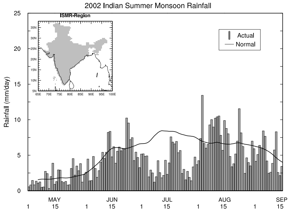
Figure 2. Daily all-India (region highlighted in the inset map) average rainfall from COLA GTS data during 2002 summer season. Daily long term mean is represented by the solid line.
