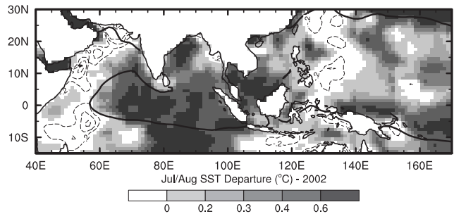
Figure 4. July–August mean SST anomaly (positive: shaded; negative: dashed contours) in 2002. Solid line highlights the region with climatological July–August mean SST greater than 28^{\circ}\text{C} .
