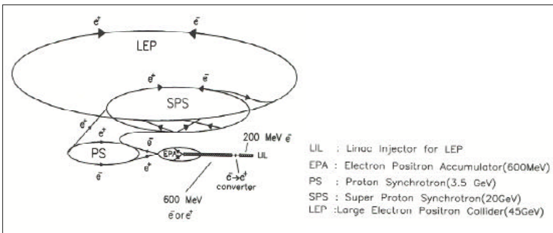
Figure 1. Acceleration of electrons and positrons for LEP.
