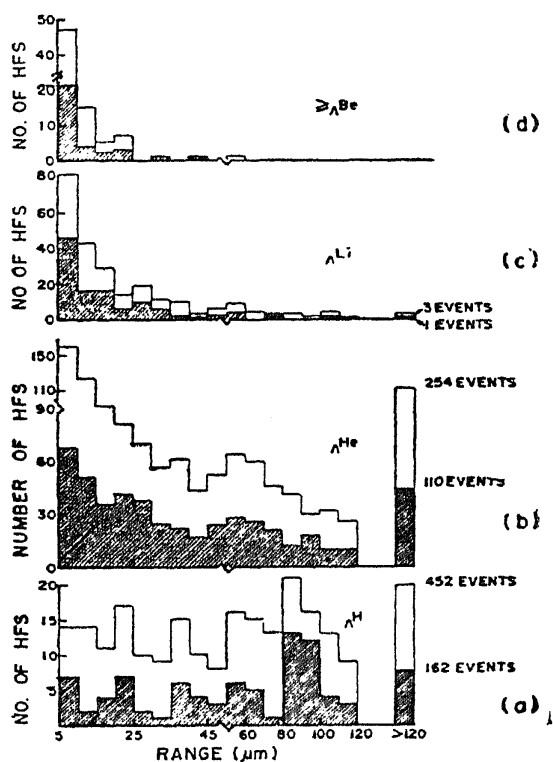
FIG. 2. (a-d) — represent the distributions of uniquely charge identified mesic HFs of range > 5\mu\text{m} and of charges 1, 2, 3 and \geq 4 respectively taken from available world raw data. The hatched histogram refers to the raw data of the present work.
