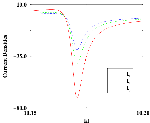
FIG. 4: Persistent current densities are plotted as function of kl . The lengths are l_1/l = l_4/l = 0.25 , l_2/l = 0.15 , l_3/l = 0.85 . Flux \phi = 0.1 .
