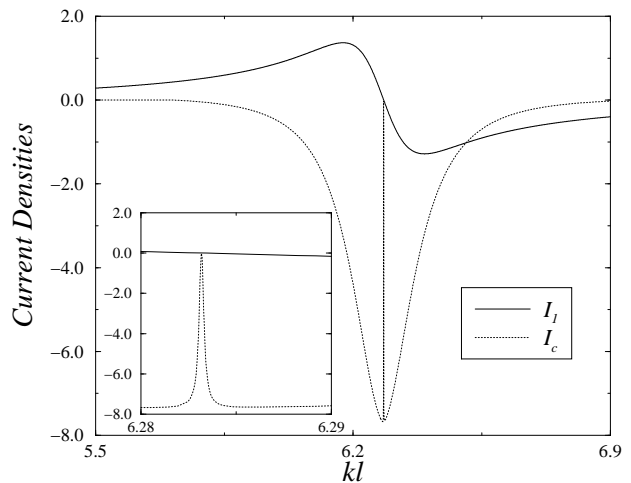
FIG. 3: Persistent current density I_1 and circulating current density I_c is plotted as function of kl . The parameters are same as used in fig. 2. The inset shows the behavior of I_c and I_1 around their zero values.
