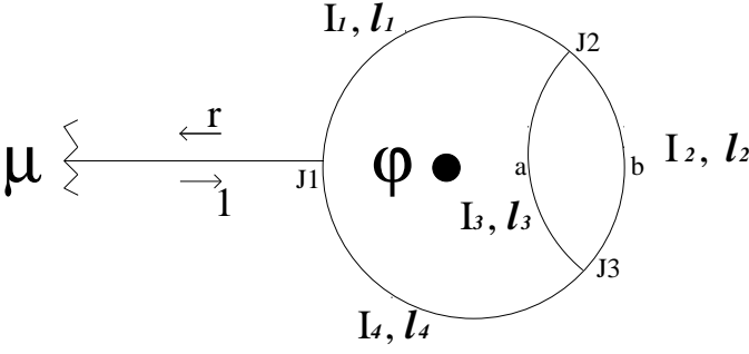
FIG. 1: One dimensional mesoscopic ring coupled to a bubble with a lead connected to a reservoir at chemical potential \mu . The localised flux \phi penetrates the ring.
