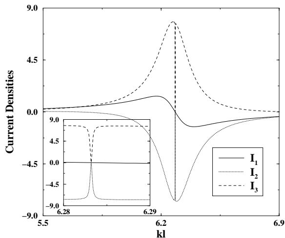
FIG. 2: Persistent current densities are shown as function of kl . The lengths are l_1/l = l_4/l = 0.25 , l_2/l = 0.45 , l_3/l = 0.55 and flux \phi = 0.1 . In the inset we have shown the current densities around the value wherein I_1 goes to zero.
