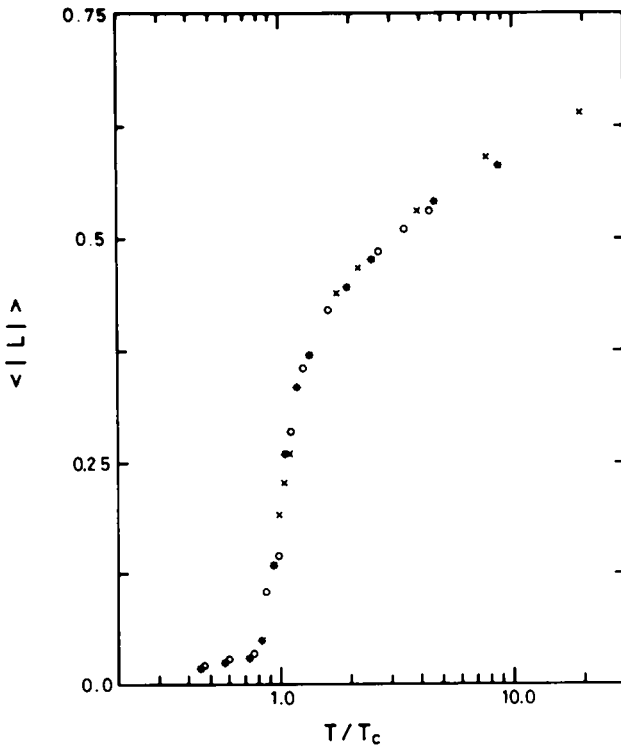
Fig. 1. Thermal Wilson loop as a function of T/T_c , calculated on a 3 \times 10^3 lattice for Wilson action ( \times ), Manton action ( * ) and Villain action ( \circ ). Here T is the temperature of the SU(2) gluon matter while T_c is the deconfinement temperature.
