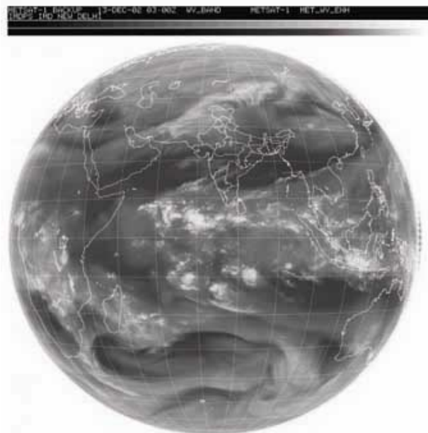
Figure 5. Water vapour imagery from Kalpana obtained on 13 December 2002.
