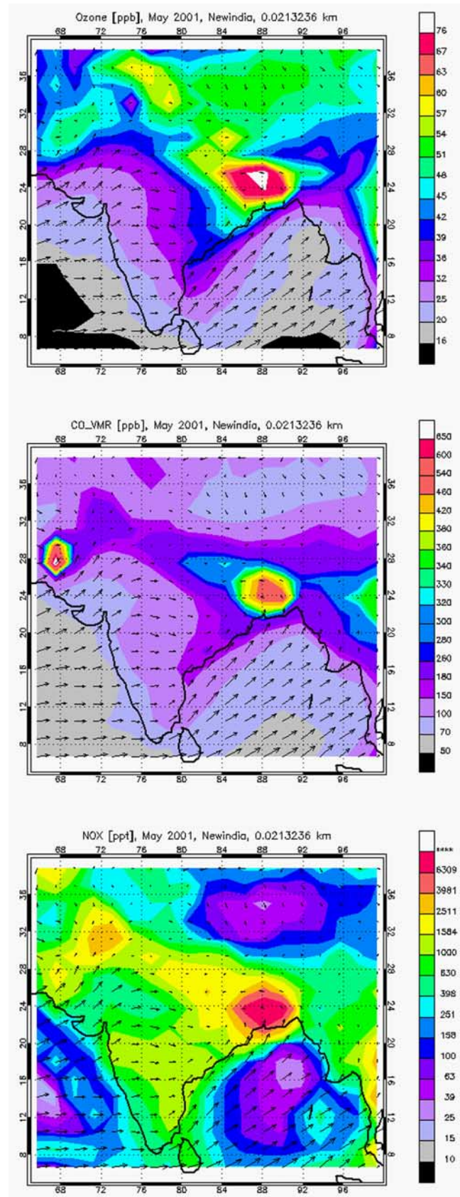
Figure 2. Distribution of \text{O}_3 (ppbv), CO (ppbv) and \text{NO}_x (pptv) at the boundary layer as simulated by MOZART for the Indian subcontinent during May (pre-monsoon season).
