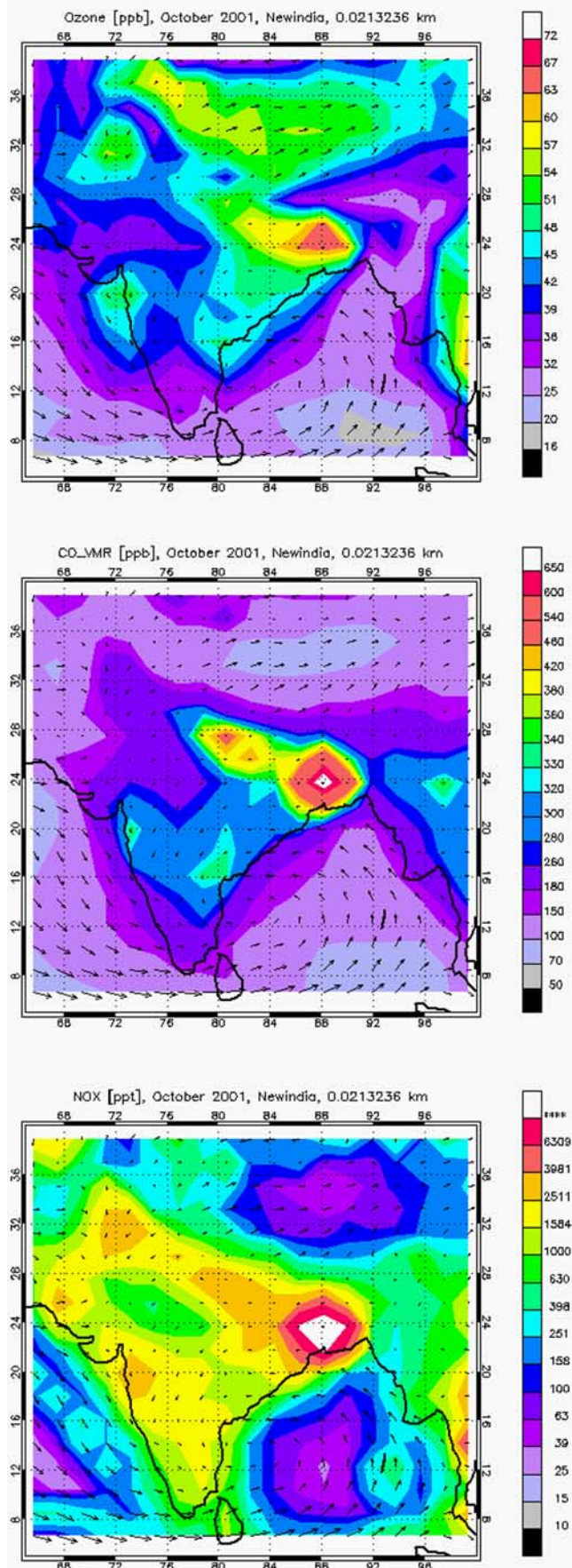
Figure 4. Same as Figure 2 but for October (post-monsoon season).
