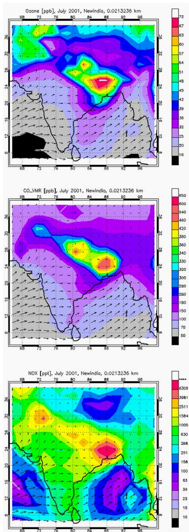
Figure 3. Same as Figure 2 but for July (monsoon season).
