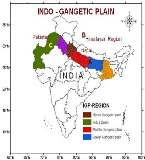
Figure 1. Geographical map showing different parts of the IGP regions (shaded area).
