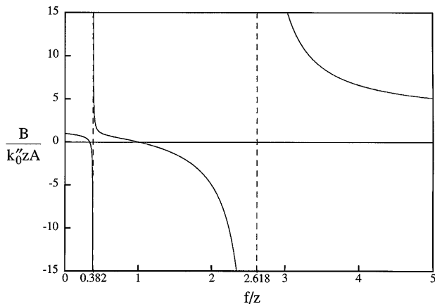
Fig. 2. Variation of the ratio B(f)/A(f) , with the focal length f for the optical system shown in Fig. 1.
