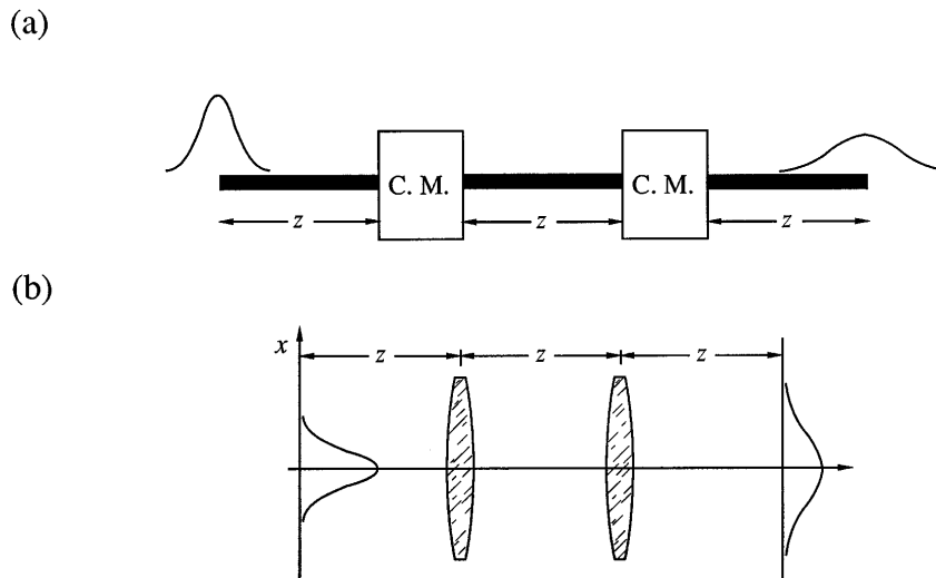
Fig. 1. Optical system used in the example of the generalized Radon transform discussed in the text. (a) The optical system for transmission of short pulses is shown symbolically with the thick lines representing lengths of a dispersive optical fiber and the chirp modulators (or time lenses) shown as blocks marked C.M. (b) The equivalent paraxial optical system for beam propagation is shown with a pair of lenses of focal length f that are separated from each other and the input and the output planes by the distance z , as shown. The lengthening of the time width of the optical pulse as it propagates through the system in (a) is mathematically analogous to the broadening of an optical beam as it is diffracted through the system in (b).
