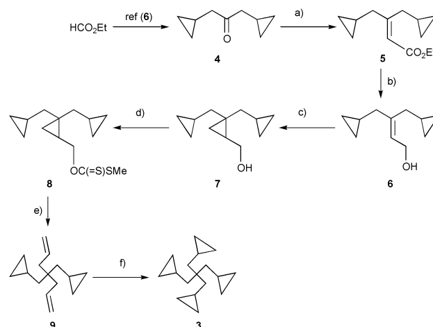
Scheme 1 Reagents and conditions: (a) (\text{EtO})_2\text{P}(\text{O})\text{CH}_2\text{CO}_2\text{Et} , NaH, THF, rt, 12 h, 62%; (b) DIBAL-H, THF, -78^\circ\text{C} , 6 h, 72%; (c) \text{Et}_2\text{Zn} , \text{CH}_2\text{I}_2 , diethyl ether, -20^\circ\text{C} , 24 h, 90%; (d) \text{CS}_2 , MeI, NaH, THF, rt, 1 h; (e) allyl \text{SnBu}_3 , AIBN, benzene, reflux, 12 h, 42% from 7 ; (f) \text{Pd}(\text{OAc})_2 , \text{CH}_2\text{N}_2 , ether, rt, 1 h, 92%.
