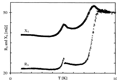
FIG. 4. R_s and X_s of HoNi_2B_2C . The AFM transition at 5.2 K is clearly visible.
