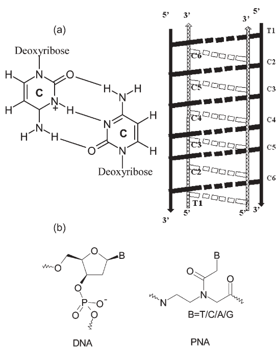
Fig. 1 (a) Schematic diagram of the i -motif in DNA. (b) Chemical structures of DNA and PNA.
