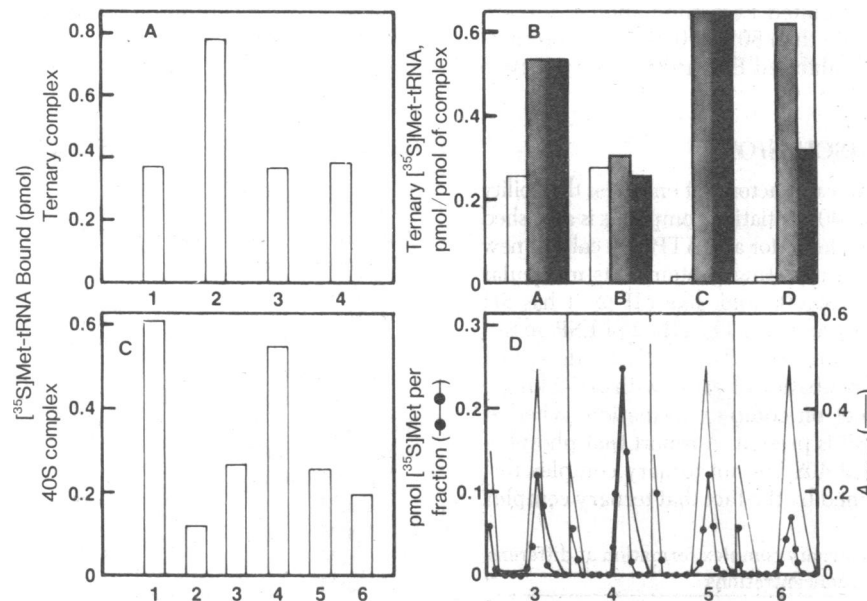
FIG. 3. Effect of ESP and inhibitor on initiation complex formation. (A) Effect on ternary complex formation. ATP (0.4 mM) and eIF-2 (6 \mu g) were present throughout. Other reactants, when present, were: ESP, 6 \mu g; inhibitor, 0.7 \mu g. Bars: 1, eIF-2; 2, eIF-2 and ESP; 3, eIF-2 and inhibitor; 4, eIF-2, inhibitor, and ESP. (B) Inhibition of ESP effect on ternary complex formation requires interaction of inhibitor and ATP with eIF-2 only. Samples (175 \mu l) containing either 35 \mu g of eIF-2 (bars A and B) or 24 \mu g of ESP (bars C and D) were preincubated with 0.057 mM ATP (bars A and C) or with 0.057 mM ATP and 3.5 \mu g of inhibitor (bars B and D) for 6 min at 30°. Other components present in all samples during preincubation were Hepes buffer, pH 7.6, 28.5 mM; Mg(OAc) 2 , 4.3 mM; KCl, 68.5 mM; and dithiothreitol, 2.8 mM. The ATP was removed with charcoal. Aliquots (35 \mu l) of the supernatant were supplemented with GTP, 0.14 mM, and [ 35 S]Met-tRNA i (25,000 cpm/pmol), 1.8 pmol, plus the following additions: In A, \square none, \blacksquare ESP (3.2 \mu g), \blacksquare ESP (3.2 \mu g) and inhibitor (0.7 \mu g); in B, \square none, \blacksquare ESP (3.2 \mu g), \blacksquare ESP (3.2 \mu g), inhibitor (0.7 \mu g), and ATP (0.04 mM); in C, \square none, \blacksquare eIF-2 (5 \mu g), \blacksquare eIF-2 (5 \mu g) and inhibitor (0.7 \mu g); in D, \square none, \blacksquare eIF-2 (5 \mu g), \blacksquare eIF-2 (5 \mu g), inhibitor (0.7 \mu g), and ATP (0.04 mM). Final volume, 50 \mu l. After incubation for 5 min at 30° the samples were assayed for ternary complex formation. The concentration of the other components present in all samples during the final incubation were: Hepes buffer, pH 7.5, 20 mM; Mg(OAc) 2 , 3 mM; KCl, 100 mM; and dithiothreitol, 2 mM. (C) Effect on 40S complex formation. Samples 1 and 2 had ESP-containing eIF-2 DE-180, 51 \mu g; samples 3–6 had eIF-2 CM-400, 18 \mu g. Other reactants, when present, were: ESP, 12 \mu g, and/or inhibitor, 2 \mu g in sample 2 or 1 \mu g in samples 5 and 6. Bars: 1, eIF-2; 2, eIF-2 and inhibitor; 3, eIF-2; 4, eIF-2 and ESP; 5, eIF-2 and inhibitor; 6, eIF-2, inhibitor, and ESP. (D) Sucrose density gradient centrifugation profiles of samples 3–6 of C.
