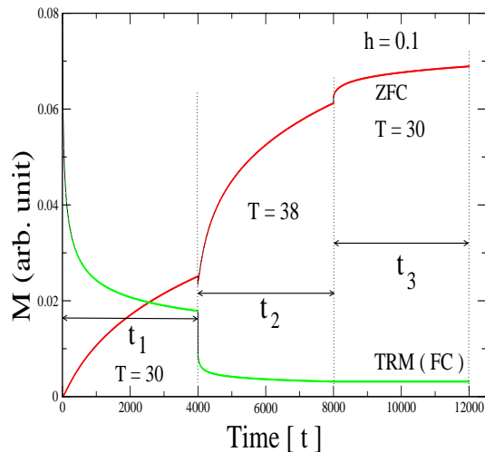
FIG. 15: (color online) Numerically simulated FC and ZFC relaxation curves with temporary heating.
