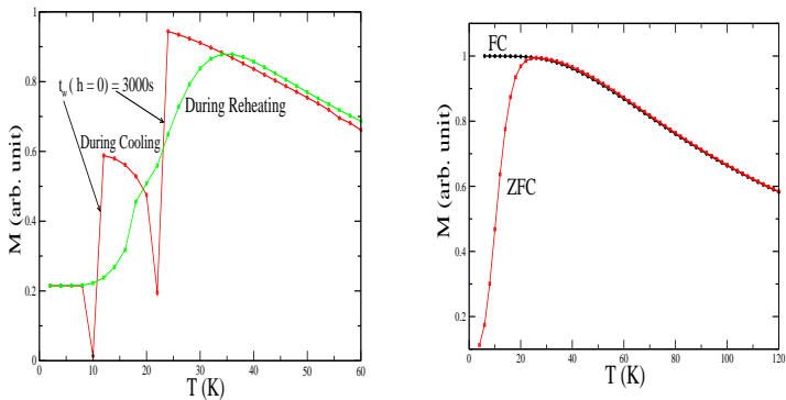
FIG. 17: (color online) (a) Numerically simulated results for the double memory experiment (DME); (b) the FCM and ZFCM vs. temperature of the interacting system are shown.
