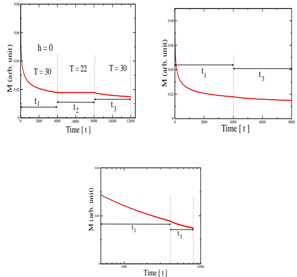
FIG. 9: (color online) (a) Numerically simulated FC relaxation curves with temporary cooling; the same data vs the total time spent at 30 K (b) on a normal scale; (c) on a logarithmic scale.
