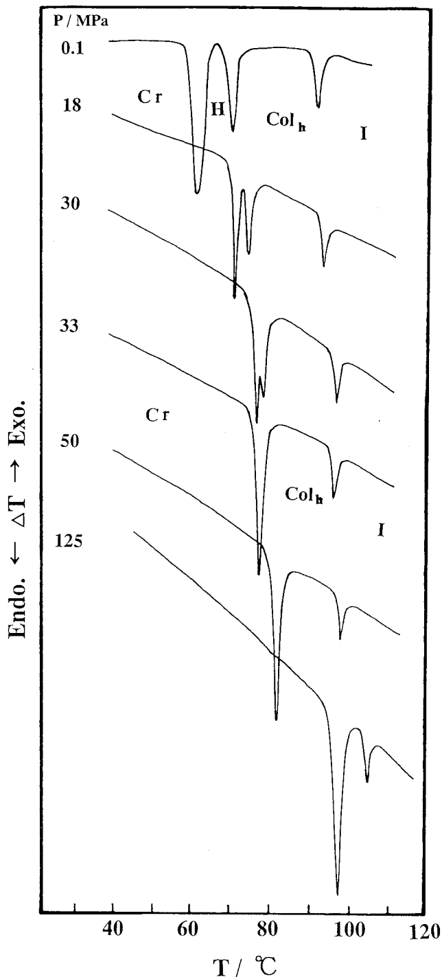
Figure 5. DTA heating curves at various hydrostatic pressures. Heating rate: 5^{\circ}\text{C min}^{-1} .
