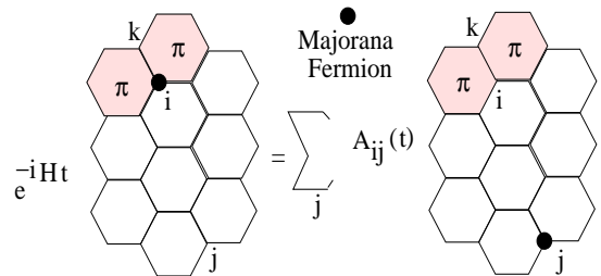
FIG. 2: Time evolution and fractionization of a spin flip at t = 0 at site i , into a \pi -flux pair and a propagating Majorana fermion. 'Shakeup' of the Majorana fermion vacuum to an instantaneous addition at t = 0 , of a \pi -flux pair is not shown.
