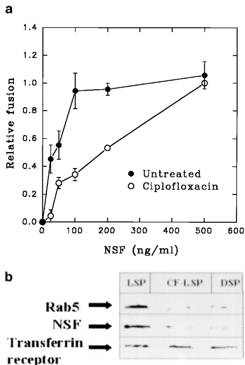
Figure 6. NSF recruitment is dependent on the presence of live Salmonella in phagosome. (a) LSP were prepared as described and treated with ciprofloxacin (500 \mu g/ml) at 4°C for 30 min. NSF on untreated and antibiotic-treated phagosomes were determined as described in Fig. 5 a. Maximum fusion obtained in LSP assay was chosen as one unit and the results are expressed as relative fusion of three independent experiments \pm SD. One unit corresponds to \sim 8.92 and 10.3 ng of HRP activity/mg of protein in the fusion assay containing live and dead Salmonella phagosomes, respectively. (b) Determination of rab5 and NSF on different Salmonella -containing phagosome. LSP and DSP were prepared as indicated and bacteria in LSP was killed by ciprofloxacin inside the phagosome (CF-LSP). Phagosomes were washed and the presence of rab5 and NSF on different phagosomes were determined by Western blot analysis using specific antibodies.
