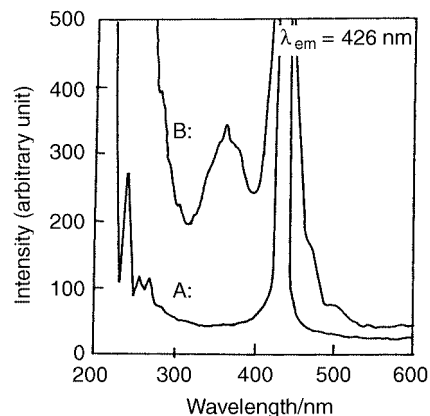
Fig. 5 Excitation spectra of (A) enediynes 6 and (B) its Ni(II)-complex at \lambda_{em} = 426 nm.
