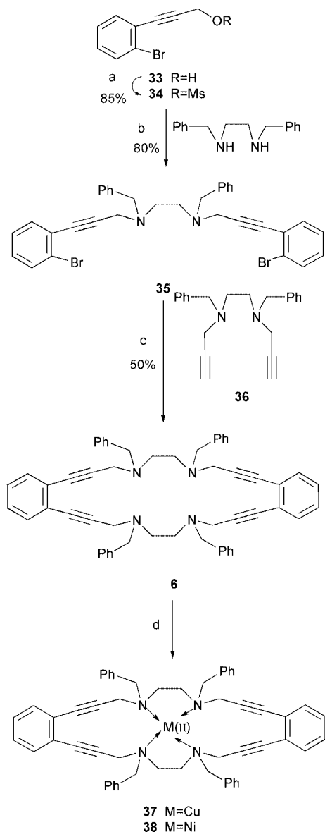
Scheme 5 Reagents and conditions: a, \text{MsCl} , \text{NEt}_3 ; b, \text{K}_2\text{CO}_3 , DMF; c, \text{Pd}(\text{PPh}_3)_4 , n\text{-BuNH}_2 , 80^\circ\text{C} ; d, \text{Cu}(\text{OAc})_2 or \text{Ni}(\text{ClO}_4)_2 , MeOH, reflux.
