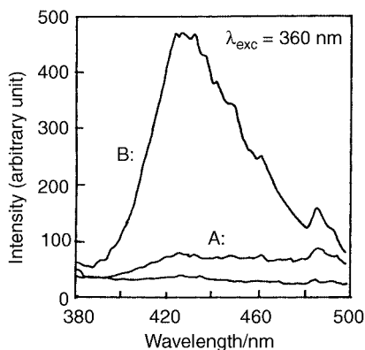
Fig. 3 Emission spectra of (A) cyclic azaenediynes 6 , (B) its Ni(II)-complex and (C) DMSO at excitation wavelength \lambda_{exc} 360 nm. Slit widths used are: excitation, 5 nm and emission, 3 nm.
