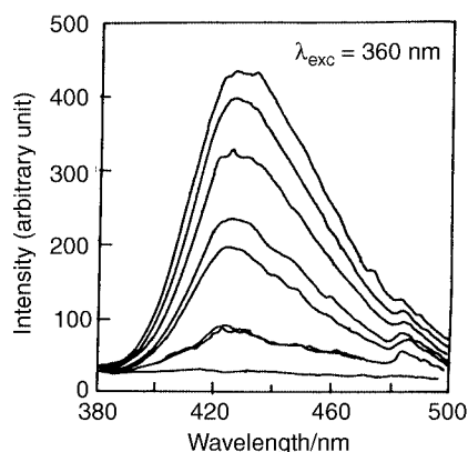
Fig. 4 Emission spectra of the Ni(II)-complex of 6 at \lambda_{exc} = 360 nm at various concentrations. (A) The topmost spectrum is for 9.0 mM concentration with each successive spectrum representing two-fold dilutions. The lowest spectrum is that of the solvent DMSO.
