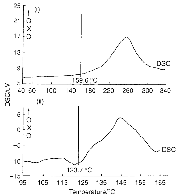
Fig. 2 DSC curve of i) tetraazaenediynes ( 6 ) and ii) its \text{Ni}(\text{II}) -complex ( 38 ).
