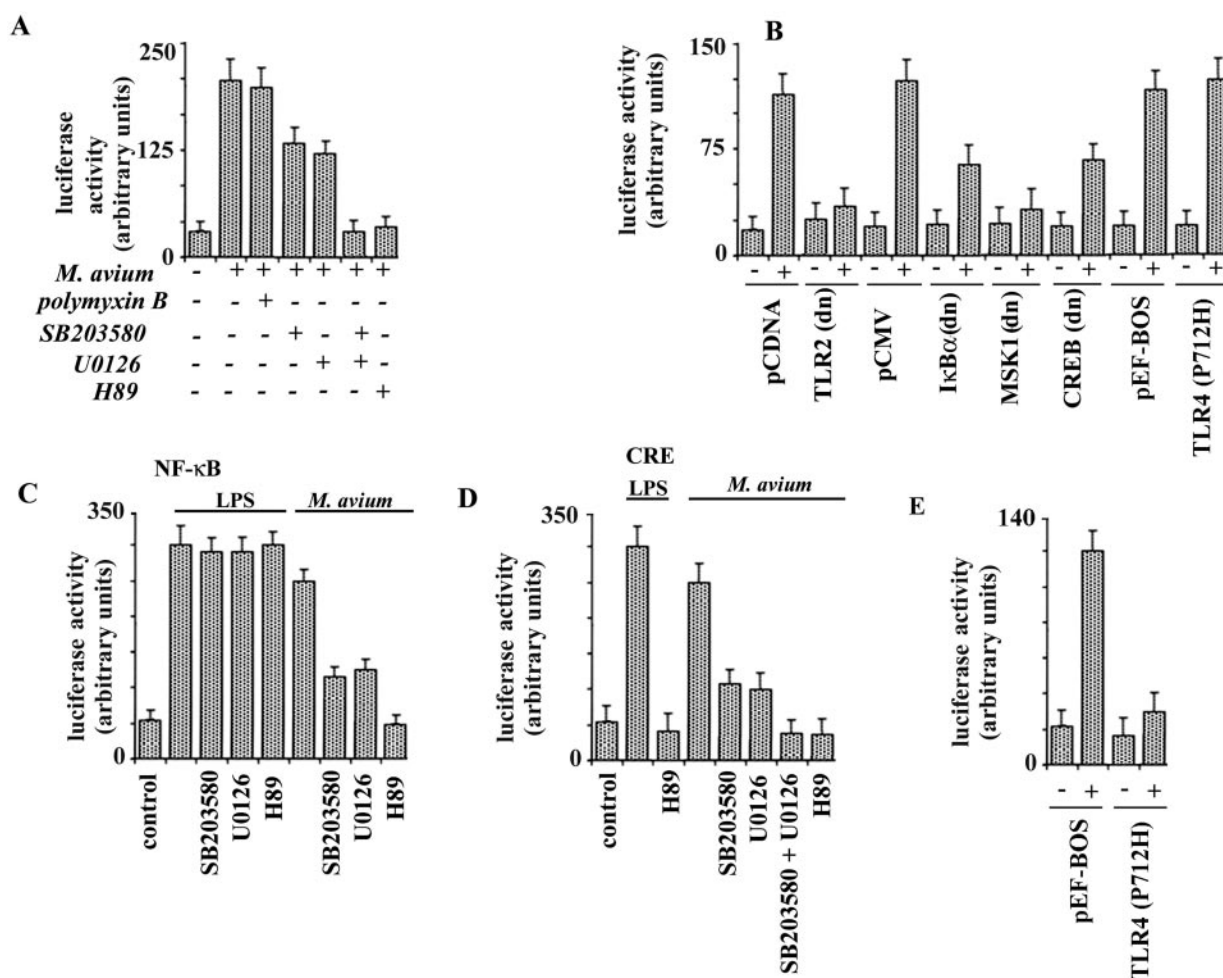
FIG. 5. M. avium stimulates COX-2 promoter-driven luciferase reporter expression in RAW264.7. RAW264.7 cells were transfected with the COX-2 promoter (-891 to +9)-luciferase reporter and \beta -galactosidase constructs. A, transfected cells were left untreated or treated with U0126 (15 \mu M), or SB203580 (5 \mu M), or H89 (10 \mu M), or a combination of U0126 and SB203580. Cells were then challenged for 6 h with M. avium or with M. avium preincubated with polymyxin B (10 \mu g/ml). In addition to the constructs mentioned above, cells were co-transfected (B and E) with empty vectors or constructs as indicated; followed by challenge with M. avium (B) or with E. coli LPS (E) for 6 h. C and D, cells were transfected with the 4 \times \kappa B-luciferase construct (C) or the 6 \times CRE-luciferase construct (D) instead of the COX-2 promoter-luciferase construct. Transfected cells were treated with inhibitors (C and D) as described above. Cells were then left untreated or incubated with E. coli LPS or with M. avium (as indicated in the panels) for 6 h. Following incubations, luciferase reporter activities in the cell extracts were measured using luciferin as substrate. In each case, the level of induction of luciferase activity was compared with that of untreated cells. The activities shown represent data that have been normalized with \beta -galactosidase activity. Results represent the means \pm S.D. of three independent experiments.
