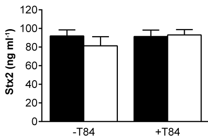
Fig. 5. Stx2 stability and T84 cell binding are not affected by oxygen levels. Purified Stx2 (100 ng ml -1 ) was incubated for 5 h with (+ T84) or without polarized T84 cells (- T84) under AE (■) or MA (□) conditions. Stx2 levels were quantified by ELISA. Data are shown as means \pm SEM from four independent experiments performed in duplicate.
