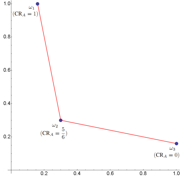
Figure 3: The three possible outcomes of the Nice or Die scenario, with the utility of agent A plotted on the horizontal axis.
