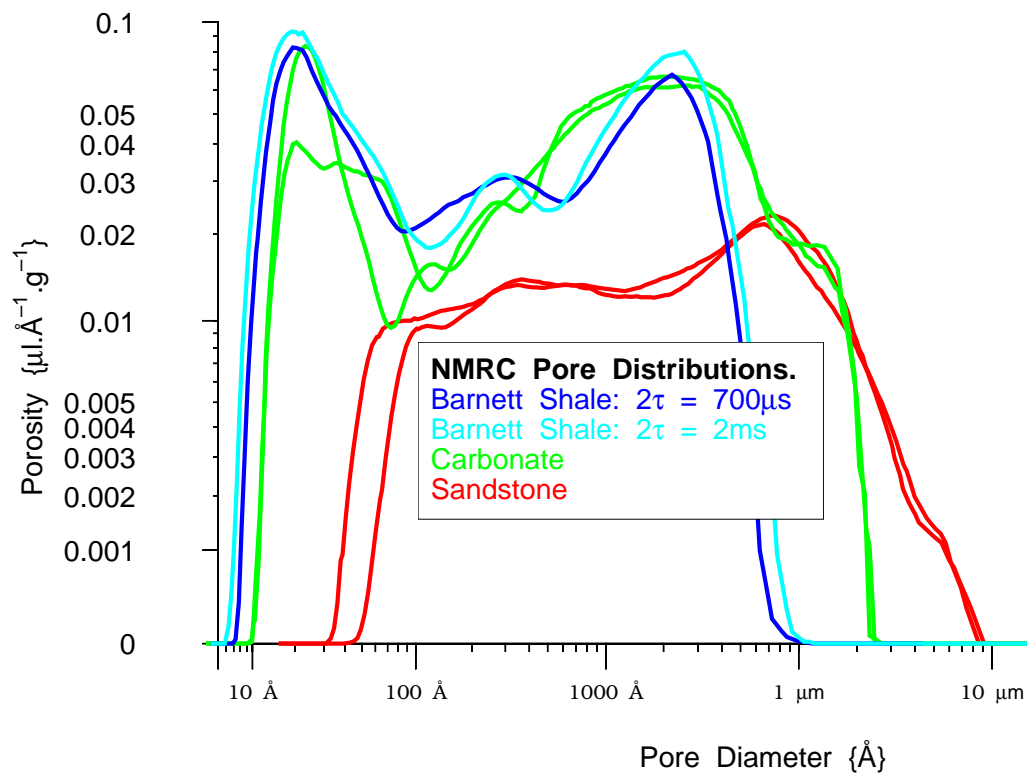
Figure 4: Measurements of open pore volume distributions in three different types of porous rock : NMR Cryoporometry (NMRC) pore-size distributions for a Barnett Shale, a Carbonate and a Sandstone, with duplicated measurements to show repeatability.
