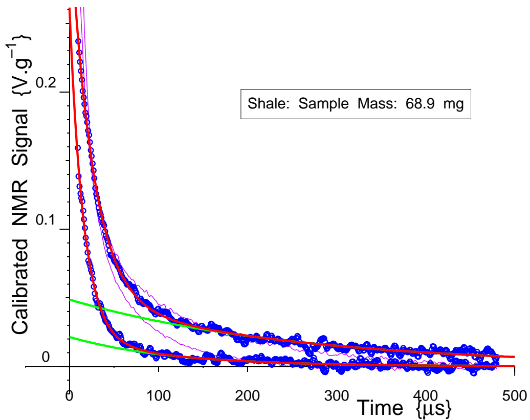
Figure 2: Two measurements of hydrocarbon quantity and dynamics/mobility in the pores of a sample of porous rock : NMR Relaxation (NMRR) Free-Induction Decays (FIDs) for organic matter in a shale, both as received (top) and after "drying" (lower). The difference is actually believed to be due to the driving off of volatile organic fractions. Also plotted (thin lines) are suitably scaled FIDs for two common road tars, for comparison.
