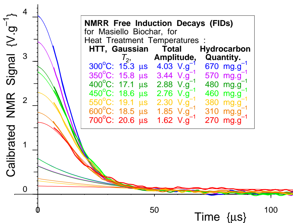
Figure 5: Measurements of hydrocarbon quantity and dynamics/mobility in the pores of biochar prepared at different HTTs : NMR Free-Induction Decays for seven biochars, with heat treatment temperatures (HTT) : 300°C, 350°C, 400°C, 450°C, 550°C, 600°C, 700°C. The samples show decreasing amplitude, in order, as increasing amounts of the labile component are driven off with higher HTT.
