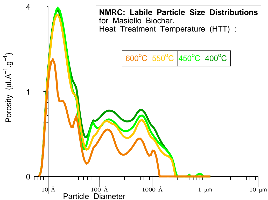
Figure 8: Particle volumes and sizes for organic fractions in biochar at a series of HTTs : NMR cryoporometric differences for four biochars, with heat treatment temperatures (HTT) : 400°C, 450°C, 550°C, 600°C; compared with the NMRC measurement for HTT 700°C. These graphs show, in order, the location and particle size distribution of the labile fraction changing, as increasing amounts of the labile component are driven off with higher HTT.
