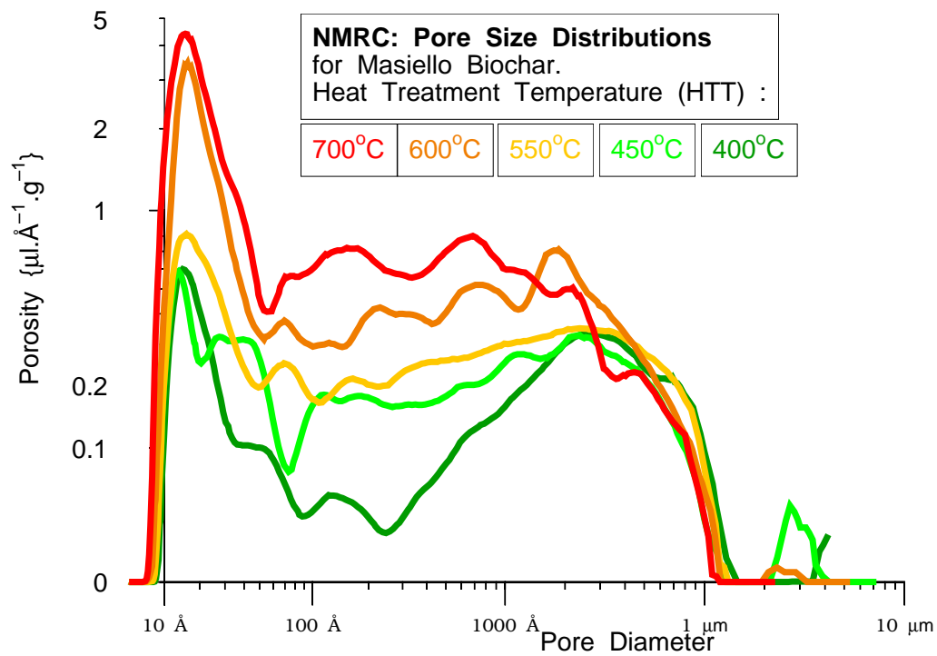
Figure 7: Measurements of open pore volume distributions for biochar prepared at five different HTTs : NMR cryoporometric measurements on five biochars, with heat treatment temperatures (HTT) : 400°C, 450°C, 550°C, 600°C, 700°C. The samples show increasing pore volumes, in order, as increasing amounts of the labile component are driven off with higher HTT.
