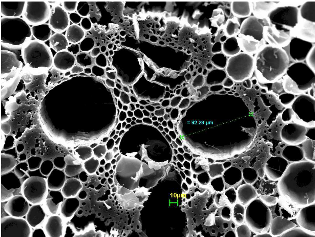
Figure 1: Microscopic structure of a Bamboo Biochar. (W.S. Teel).
