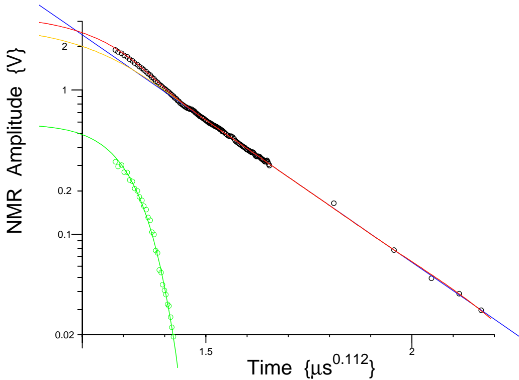
Figure 3: Extraction of fit parameters for tars, to compare with organic fractions in shale: Fitted NMR Free-Induction Decays and CPMG data for a common road Tar. Straight line : stretched-exponential fit to measured data in region x = 1.5 to 2.2 \mu s^{0.112} . Curve through y=2 : equivalent exponential distribution fit in same range. Lower circles : residual difference, with a Gaussian fit.
