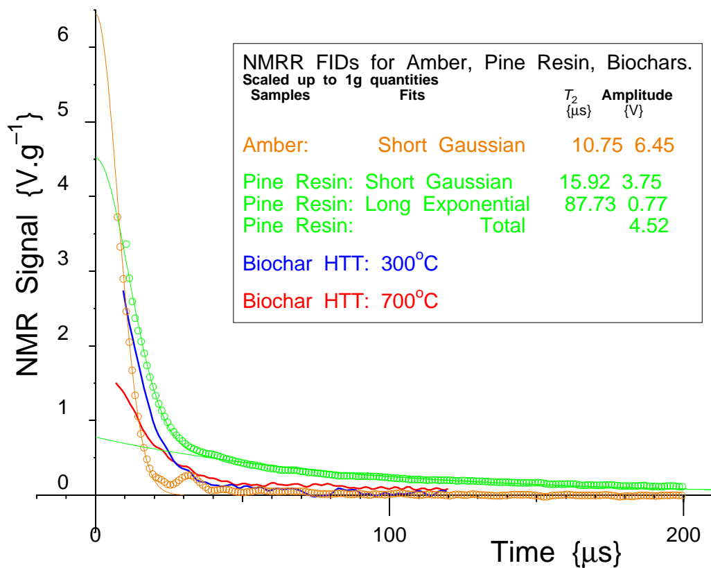
Figure 6: NMR Free-Induction Decays for Amber (upper circles) and fresh Pine Resin (lower circles), compared with two biochar with heat treatment temperatures (HTT) : 300°C and 700°C (thick lines).
