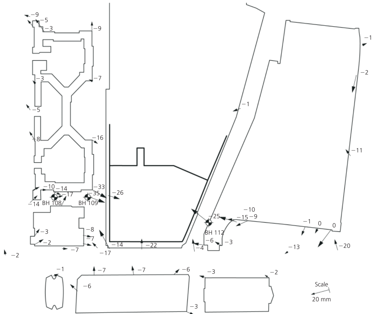
Figure 5. Displacement at ground surface to end of excavation in 1987. Numbers represent settlements in mm; arrows show displacements in plan
