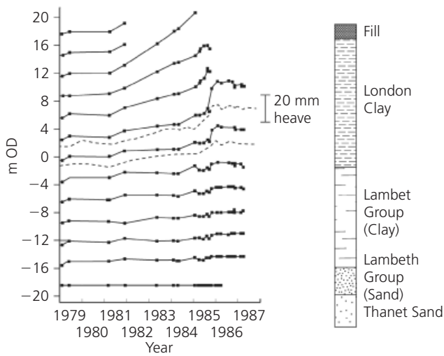
Figure 21. Extensometers 120 (solid lines) and 122 (broken lines)
