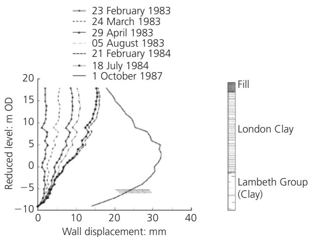
Figure 12. Inclinometer F75
