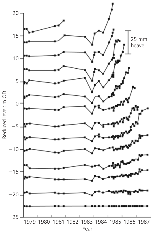
Figure 17. Extensometer 117 in the south area
