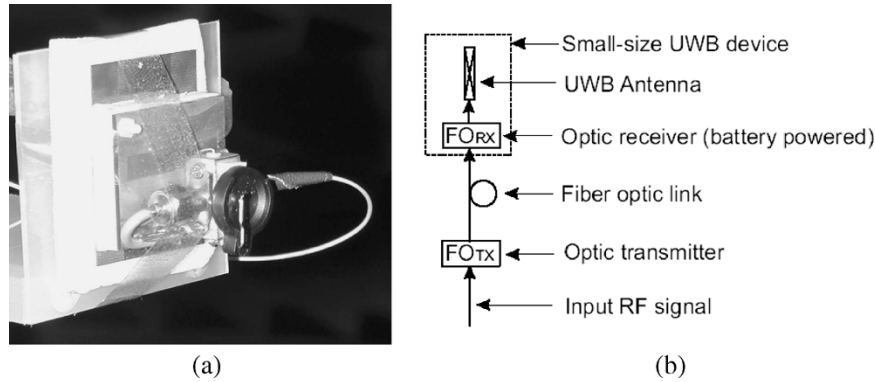
Fig. 1. Small-size antenna measurement setup using RF on fiber optic: (a) photo of the antenna measurement setup (antenna, optical receiver and fiber link) and (b) block diagram of the RF on fiber optic setup.
