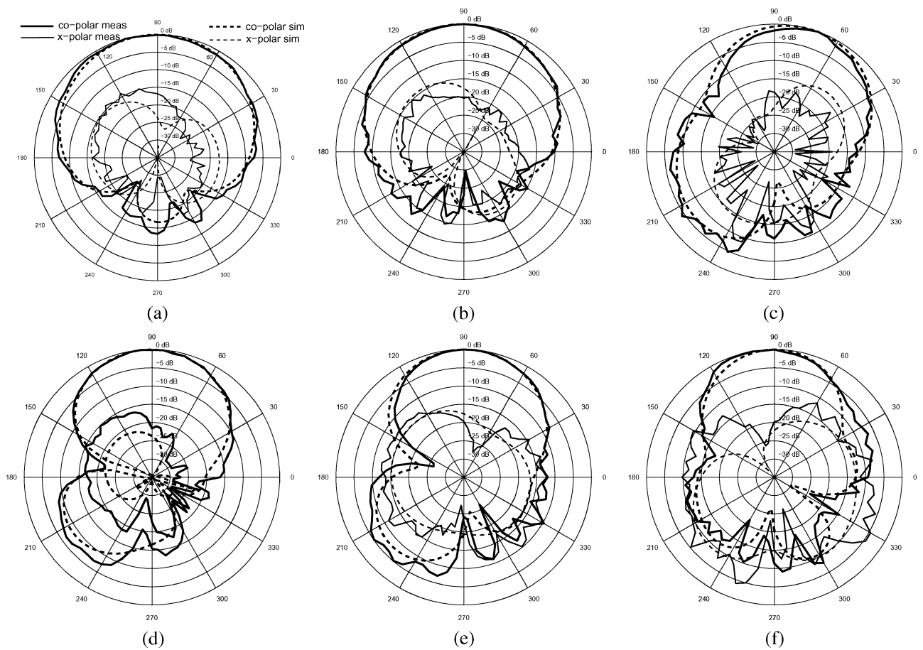
Fig. 2. Comparison of measured and simulated radiation patterns of directional slot antenna [see Fig. 1(a)]. (a) XZ plane 3.5 GHz, (b) XZ plane 4.5 GHz, (c) XZ plane 6 GHz, (d) YZ plane 3.5 GHz, (e) YZ plane 4.5 GHz, (f) YZ plane 6 GHz.
