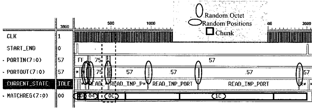
Figure 3: Cipher text randomization
