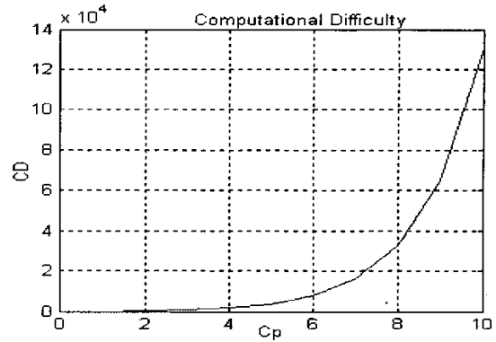
Figure 8: Computational difficulty
