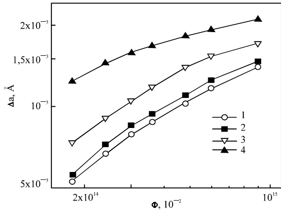
Fig. 1: Dependence of the Silicon Lattice Constant \Delta a_s on B^+ Ion Fluence \Phi in: -Si:P, \rho_0 = 0.5 \Omega \text{ cm} ; (2-4)-Si:B, \rho_0 = 0.005 \Omega \text{ cm} ; j_{ef} : (1,3)-0.2; (2) - 0.5; (4)-0.05 \mu\text{A cm}^{-2}
