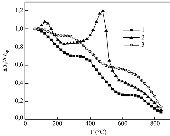
Fig. 2: Lattice Constant Recovery at Isochronal 15 min Annealing of Implanted Silicon. \Delta a_\Phi -Change of Lattice Constant after Ion Implantation with Fluence \Phi ; \Delta a_T -Change of Lattice Constant after Ion Implantation and Annealing at Temperature T.-Si:P, \rho_0 = 0.5 \Omega \text{ cm} ; (2)-Si:B, \rho_0 = 0.005 \Omega \text{ cm} ; (3)-Si:B, \rho_0 = 0.005 \Omega \text{ cm} , Annealing with Electron Illumination
