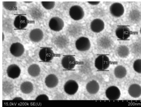
Fig. 7. – The SEM picture of the nanoporous alumina sample from a surface.
