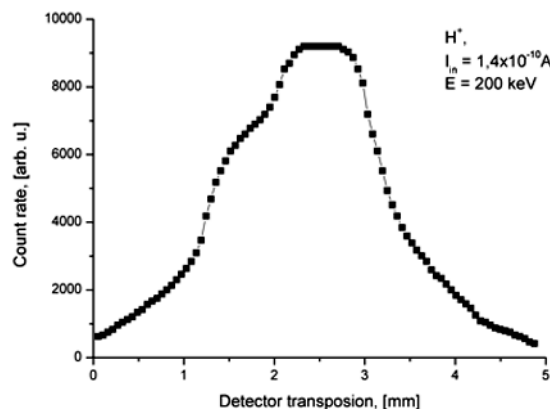
Fig. 4. – Shape and angular distribution of 200 keV protons transmitted through a capillary with a taper angle of 0.5 deg.
