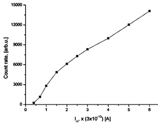
Fig. 2. – Count rate of particles transmitted through the capillary vs. proton current at the input of the capillary.
