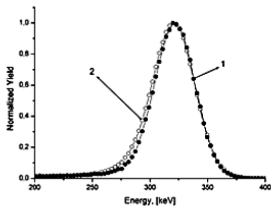
Fig. 6. – Energy spectrum of transmitted protons with an initial energy of 320 keV with and without capillary. The taper angle is 1.7 deg. Curve 1 is for the initial beam and curve 2 is for the transmitted beam.
