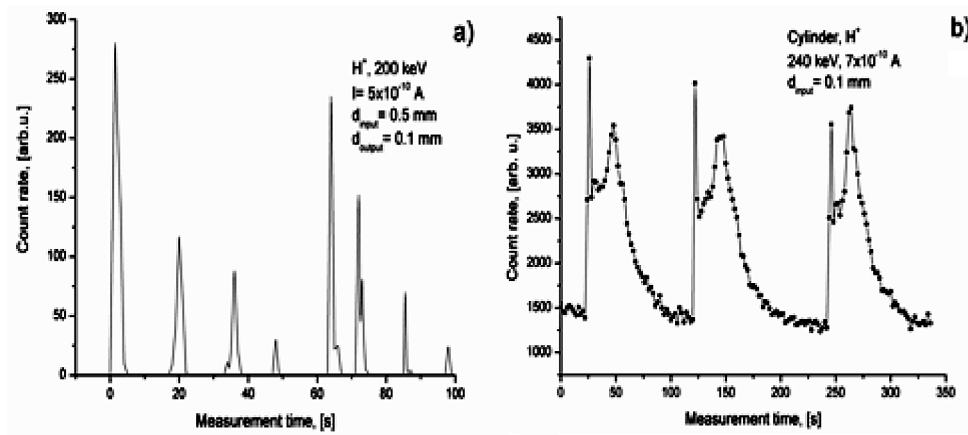
Fig. 3. – Time distributions of protons transmitted through a tapered capillary (a) and cylindrical capillary (b).
