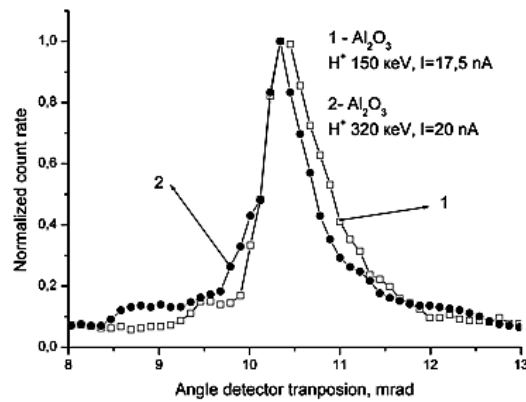
Fig. 9. – Angular distribution of H^+ ions transmitted through capillaries in the Al_2O_3 membrane without metallic coverage at 0^\circ tilt angle: 1–150 keV, I = 17.5 nA; 2–320 keV, I = 20 nA.
