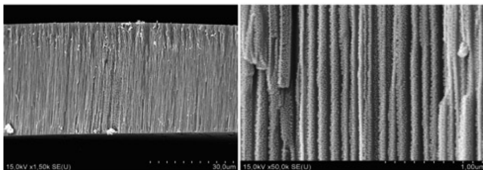
Fig. 8. – The SEM image of a side view of the nanoporous alumina sample at different magnifications.
