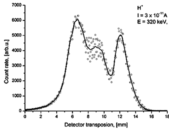
Fig. 5. – Angular distribution of 320 keV protons transmitted through a capillary with a taper angle of 2.2 deg.
