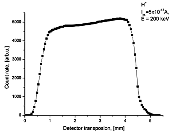
Fig. 1. – Shape and angular distribution of a 200 keV proton beam transmitted through the capillary.
