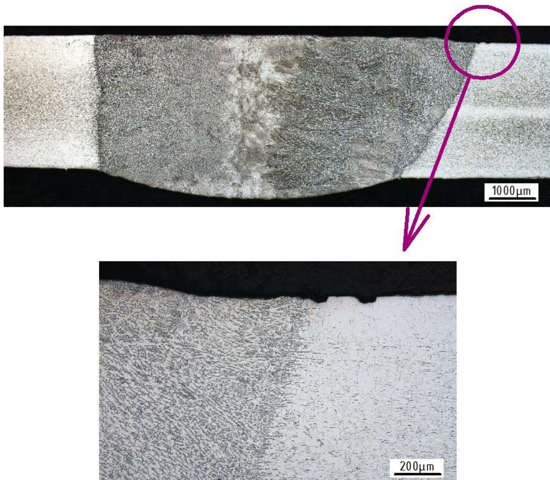
Fig. 5. Corrosion attack of the specimen with untreated surface.
