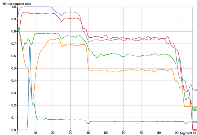
Figure 5.19: Flash disconnect scenario: hit/request-ratio for different stratum buckets (0-20 blue, 21-40 orange, 41-60 green, 61-80 red, 81-100 purple) when simulating 100 peers.
