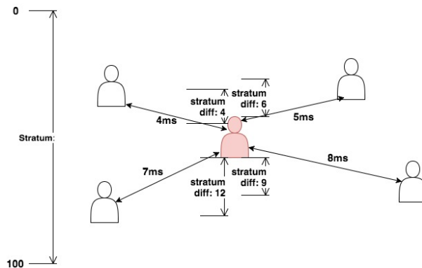
Figure 2.6: The peer in red, and its neighbours in white. Considers latency and stratum difference when determining its best candidates.
