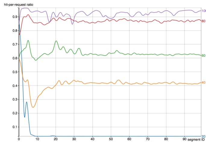
Figure 5.3: Optimal scenario: hit/request-ratio for different stratum buckets (0-20 blue, 21-40 orange, 41-60 green, 61-80 red, 81-100 purple) when simulating 1000 peers.
