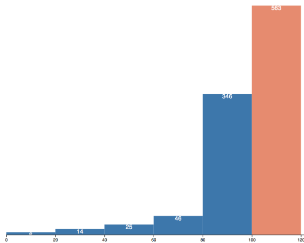
Figure 5.24: Flash disconnects scenario: histogram for the number of peers in the different stratum buckets (101-120 are disconnected peers) 3 minutes after the flash disconnects, when simulating 1000 peers.
