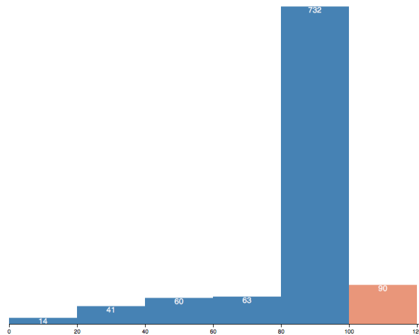
Figure 5.10: Default scenario: histogram for the number of peers in the different stratum buckets (101-120 are disconnected peers) at the 50th segment, when simulating 1000 peers.
