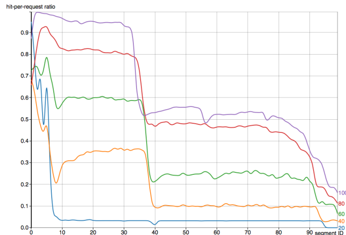
Figure 5.20: Flash disconnect scenario: hit/request-ratio for different stratum buckets (0-20 blue, 21-40 orange, 41-60 green, 61-80 red, 81-100 purple) when simulating 1000 peers.
