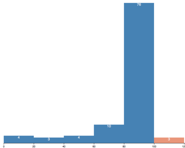
Figure 5.9: Default scenario: histogram for the number of peers in the different stratum buckets (101-120 are disconnected peers) at the 50th segment, when simulating 100 peers.
