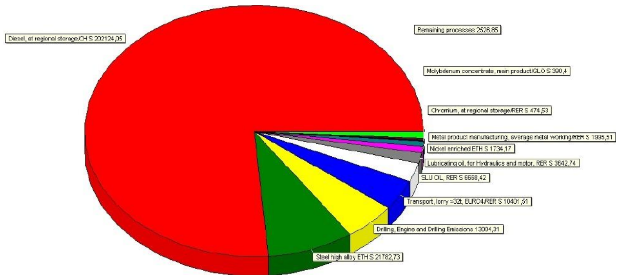
Figure 14 - Environmental impacts of Sandvik Mining DX780 Drill Rig Source: Rouhiainen (2008)
