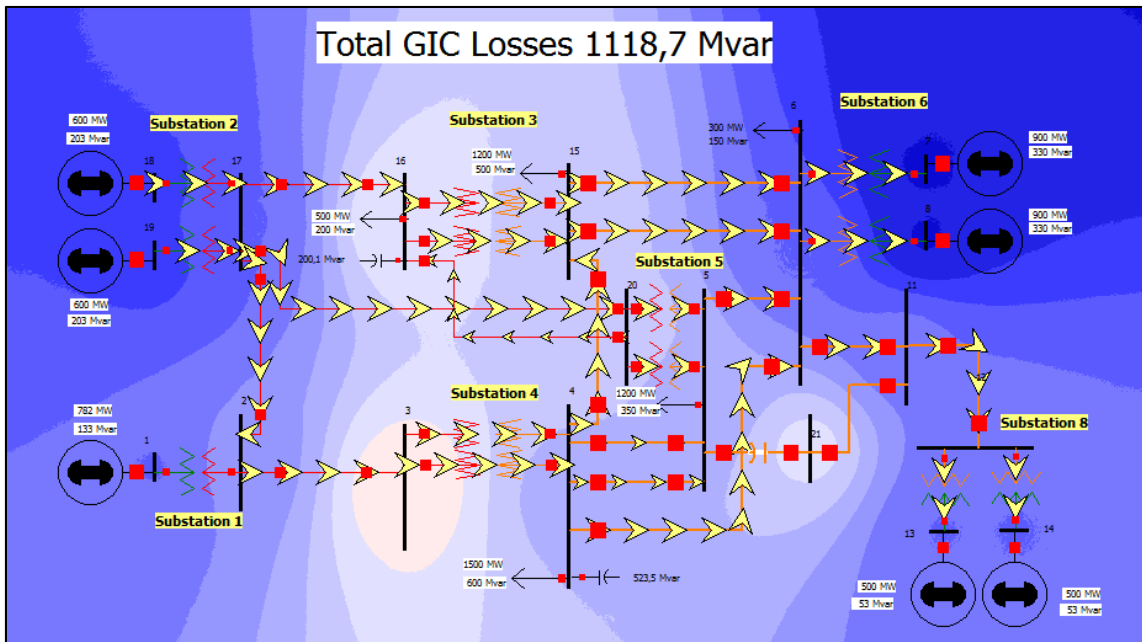
Figure 38 21 Bus system without two of the transformers in parallel.
