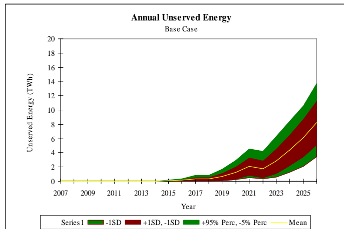
Figure 39: Annual Unserved Energy for Base Case
