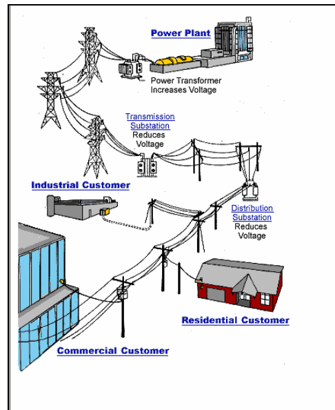
Figure 14: Example of an electricity network 64
