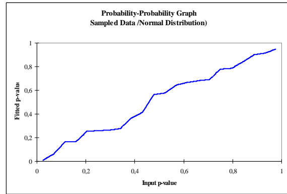
Figure 35: Probability -Probability Graph, Sampled data versus Fitted Distribution
