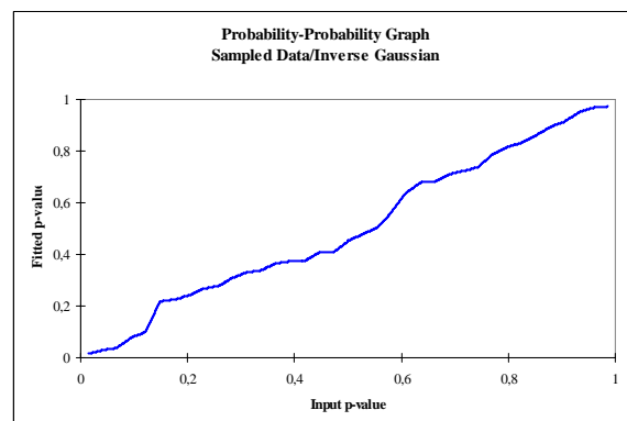
Figure 30: Probability-Probability Graph, Sampled data versus Fitted Distribution
