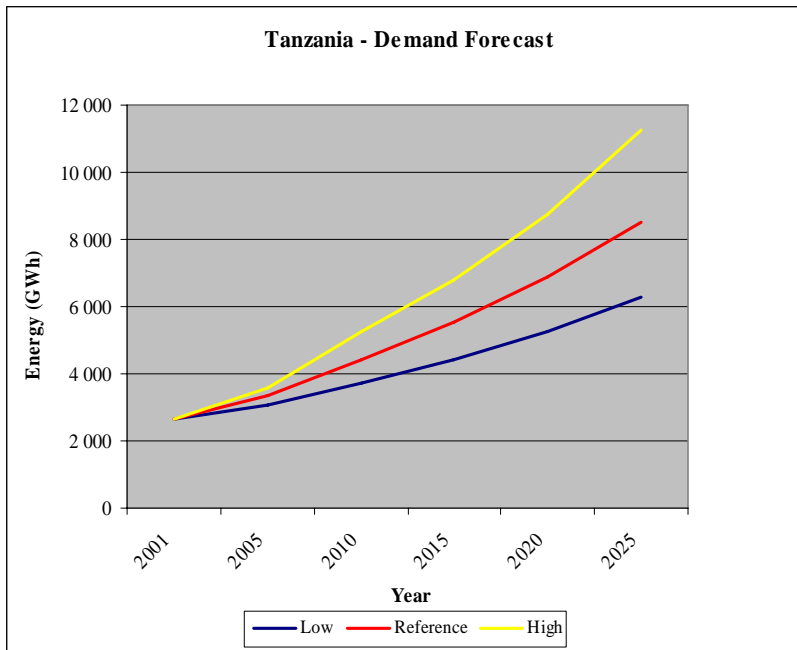
Figure 20: Demand Forecast – 3 Scenarios of EAPMP
