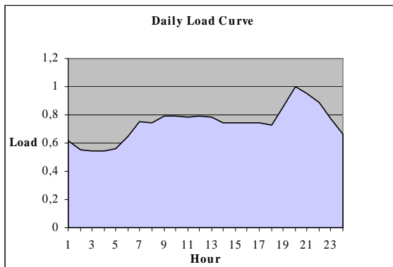
Figure 10: Typical Daily Load Variations 55
