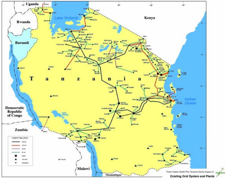
Figure 16: TANESCO's Transmission System
