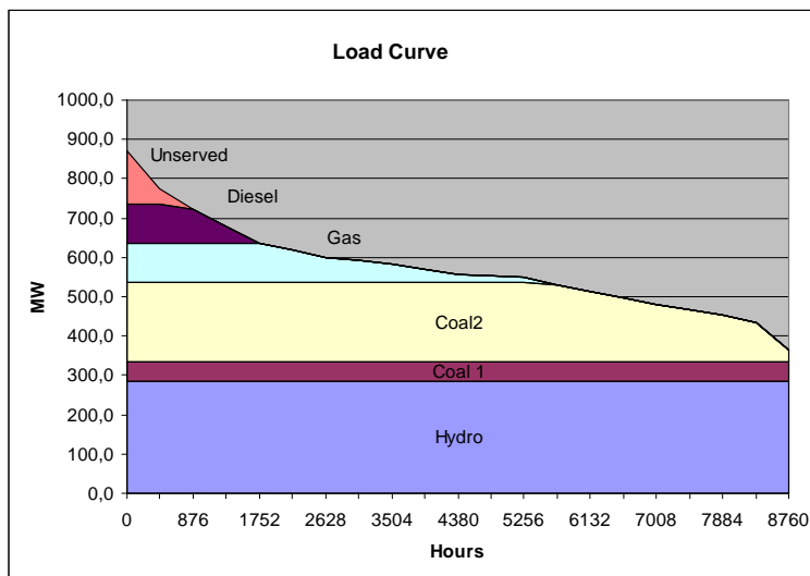
Figure 23: Example of a Load Curve for Tanzania's Power System
