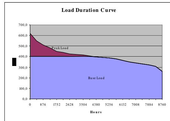
Figure 11: Load Curve Diagram
