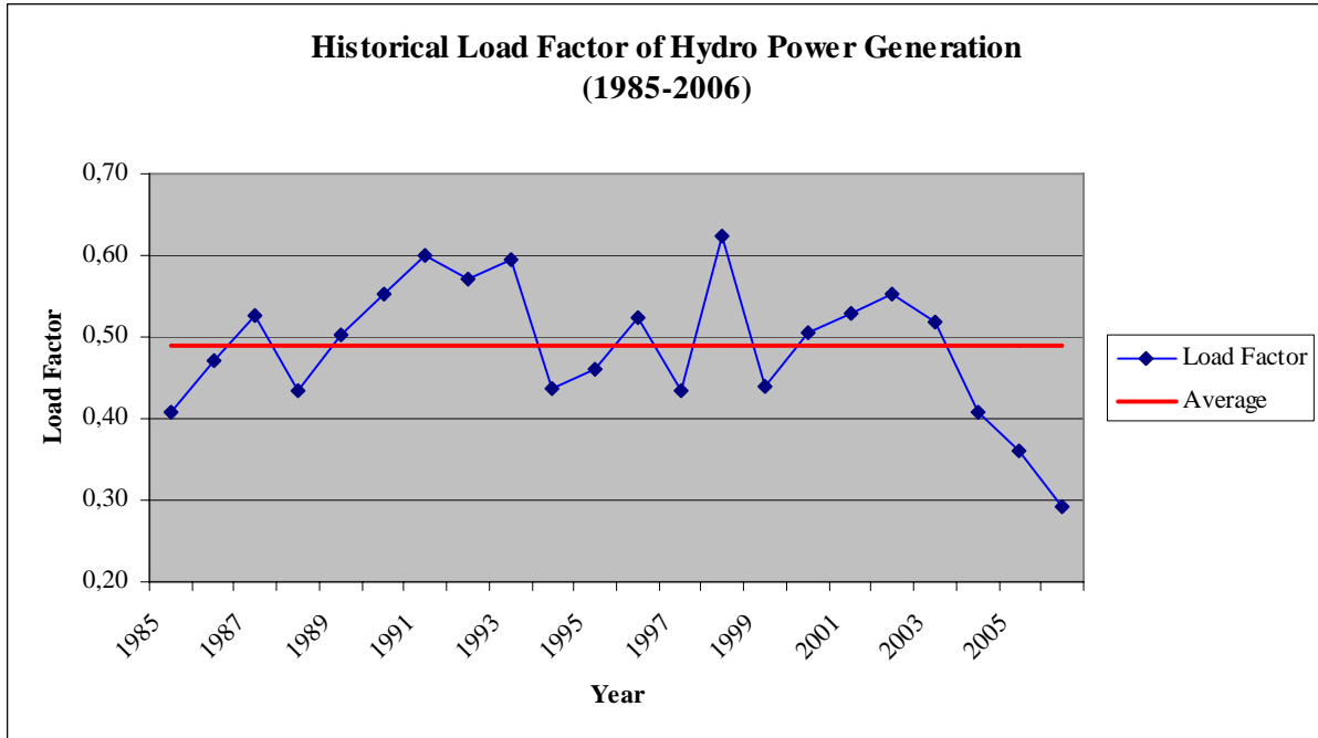
Figure 33: Historical Load Factor of Hydro Power Generation
