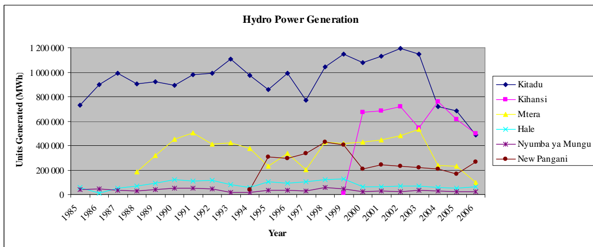
Figure 32: Generated units of Energy from TANESCO's Hydro Power Stations
