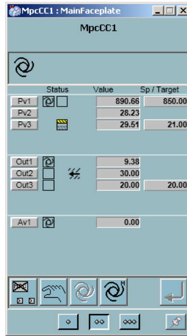
Figure C.2 The main faceplate in standard view mode.
