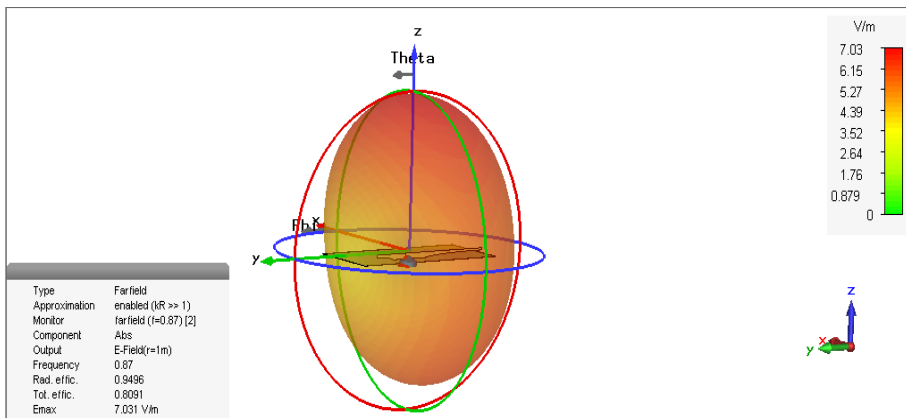
Fig. 4.24: T-strip antenna radiation pattern in the high band
