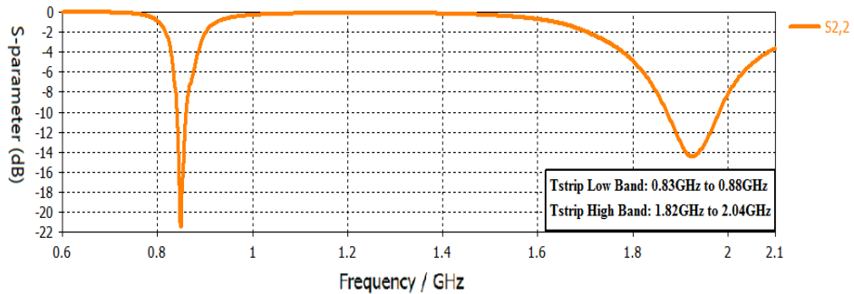
Fig. 4.21: Reflection coefficient of the T-strip antenna
