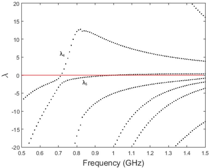
Fig. 2.4: Eigenmodes of a rectangular plate with a half-bezel structure
