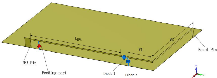
Fig. 4.10: Compressed IFA/bezel Reconfigurable Antenna Single Band Design
