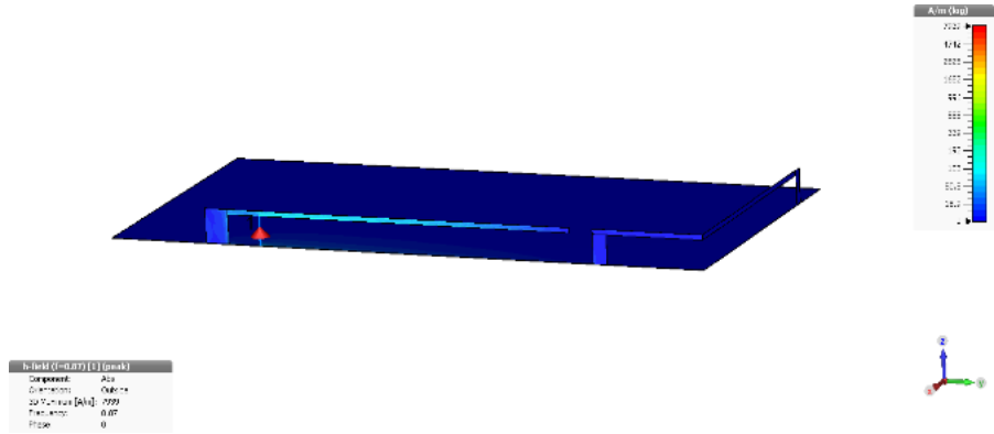
Fig. 4.12: IFA state current distribution
