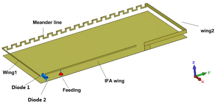
Fig. 4.2: IFA/bezel reconfigurable antenna design
