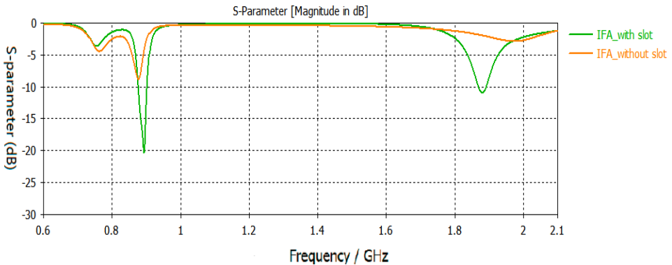
Fig. 4.18: Reflection coefficients for the IFA state with/without slot
