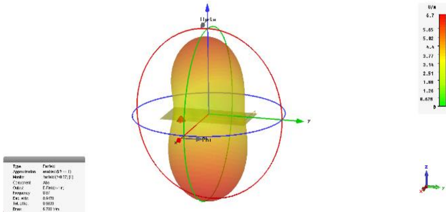
Fig. 4.15: Bezel state radiation pattern
