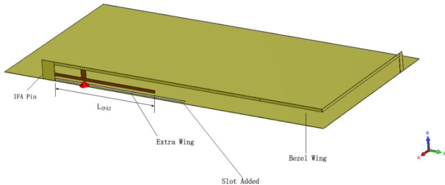
Fig. 4.16: Extra wing added in the bezel state for dual-band resonances
