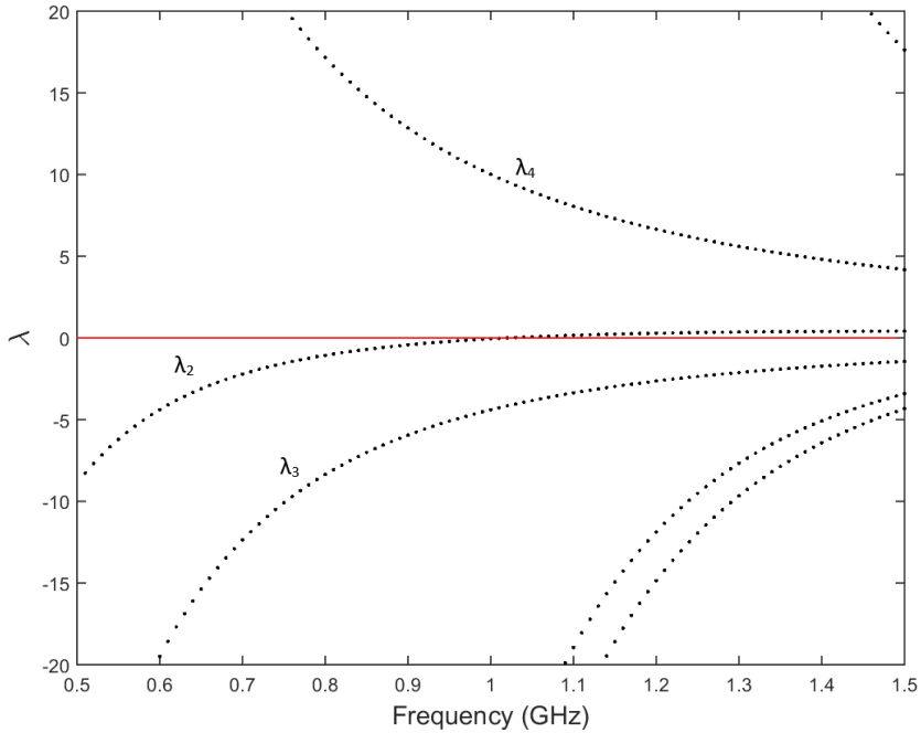
Fig. 2.1: Eigenmodes of a rectangular plate from 0.5 GHz to 1.5 GHz
