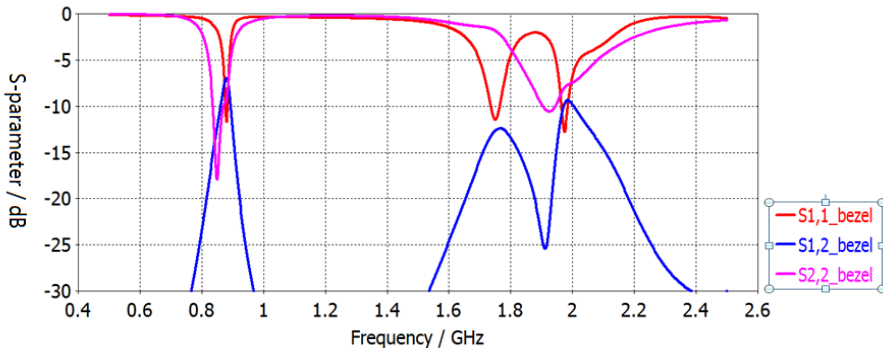
Fig. 5.4: S parameters of the final structure in the IFA state
