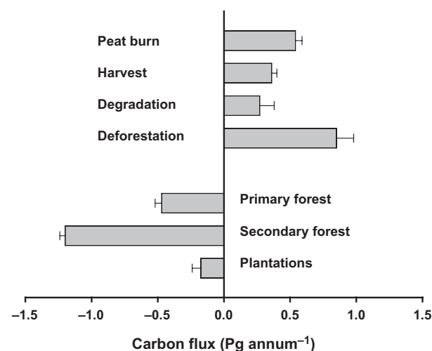
Fig. 4 Components of human-induced change in the tropical biological carbon balance, with uncertainties. Negative denotes uptake from the atmosphere to the land surface, positive denotes loss of carbon to the atmosphere. The data are applicable to the period 2005–2010.
