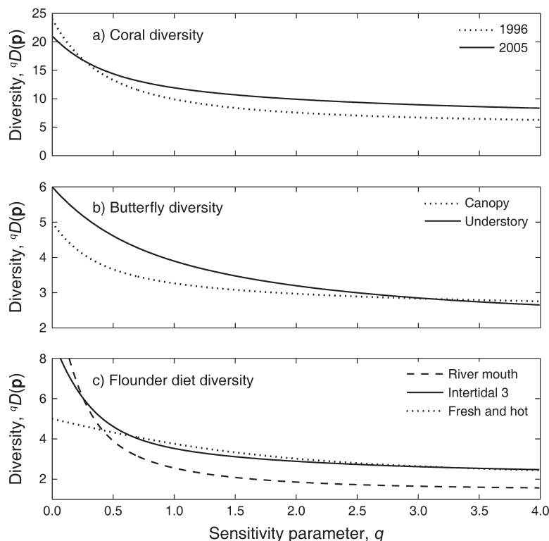
FIG. 2. Diversity profiles using naive similarity matrix: (a) Coral (data from Table 4 of Riegl et al. [2009]); (b) butterflies of subfamily Nymphalinae (data from Table 5 of DeVries et al. [1997]); (c) flounder diet (data from Wirjoatmodjo [1980]).
