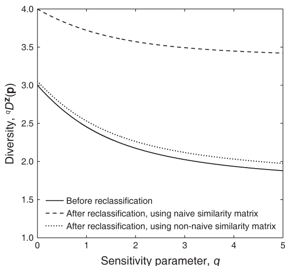
FIG. 1. Diversity profiles of a hypothetical community, before and after taxonomic reclassification.
