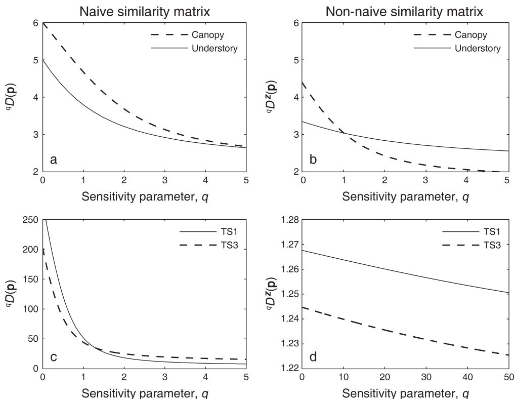
FIG. 3. Illustration of different similarity matrices: diversity profiles of six butterfly species of subfamily Charaxinae (with an abundance table) using (a) the naive similarity matrix, and (b) a taxonomic similarity matrix (data from DeVries et al. [1997: Table 5]). The bottom two panels show diversity profiles of the gut microbiomes in a lean child (TS1) and an overweight mother (TS3) (Turnbaugh et al. 2009), using (c) naive and (d) genetic similarity matrices. Note the different scales.
