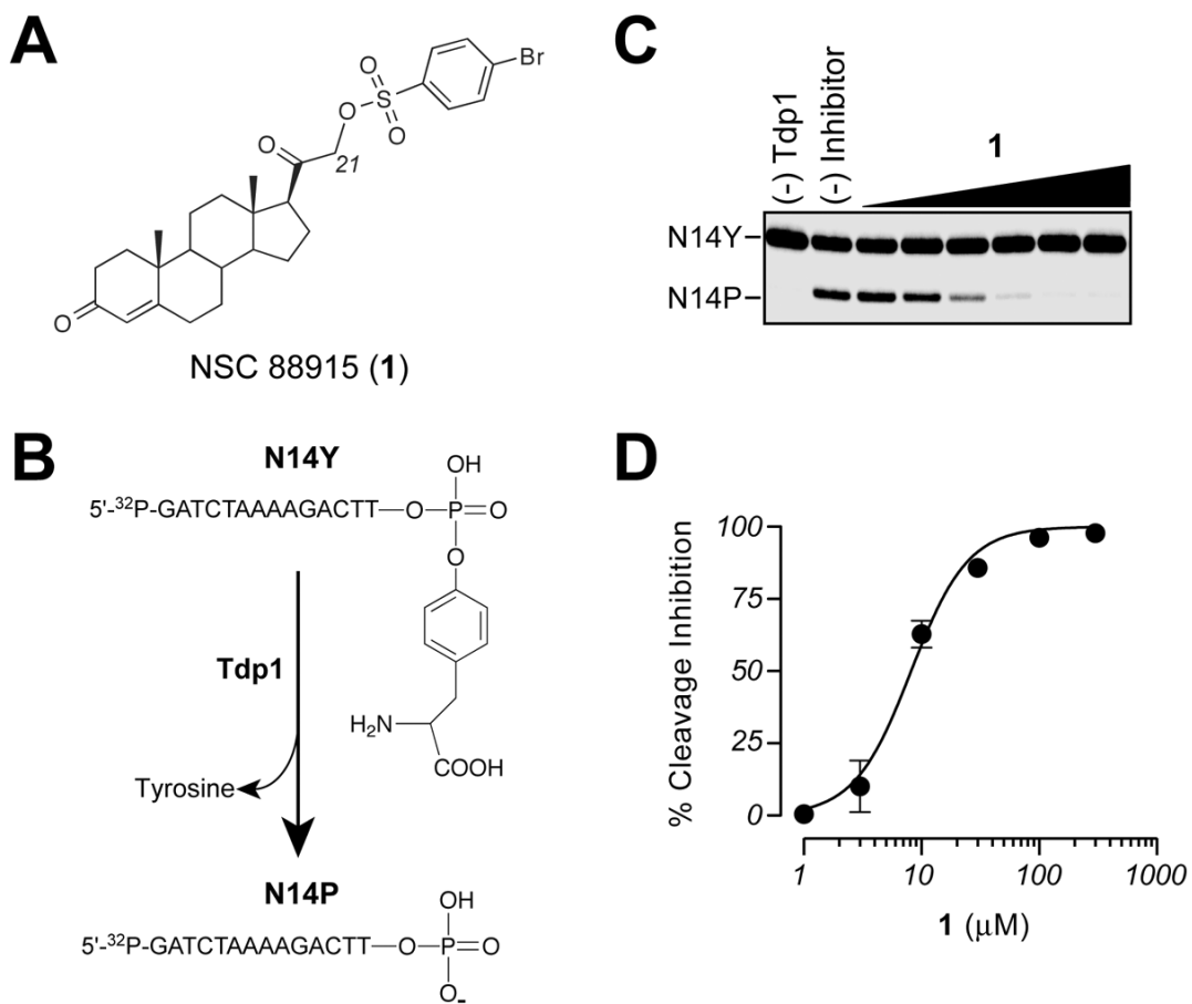
Figure 1. Tdp1 inhibition by 1 . A) Chemical structure of 1 . B) Schematic representation of the Tdp1 gel-based biochemical assay. Tdp1 hydrolyzes the 3'-phosphotyrosine bond and converts N14Y to an oligonucleotide containing a 3'phosphate (N14P). C) Representative gel demonstrating dose-dependent inhibition of Tdp1 by 1 . D) Graphical representation of the percent inhibition of Tdp1 by 1 . Each point represents the mean \pm SEM for three independent experiments.
