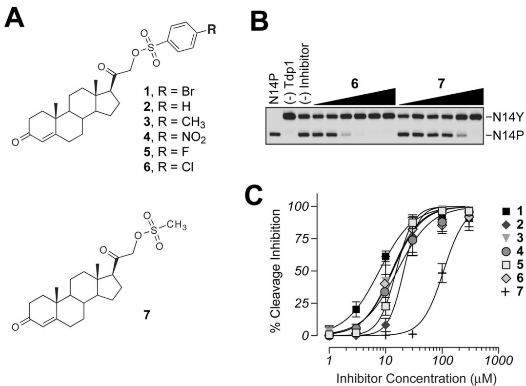
Figure 4. Structure-activity relationship of analogues of 1 . A) Chemical structures of the analogues tested. B) Representative gel demonstrating dose-dependent inhibition of Tdp1 by 6 and 7 . C) Graphical representation of the percent inhibition of Tdp1 by 1–7 . Each point represents the mean \pm SEM for three independent experiments.
