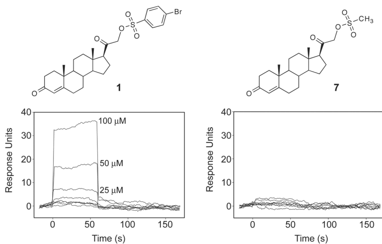
Figure 6. Differential binding of 1 and 7 to Tdp1 using surface plasmon resonance (SPR). SPR sensorgrams showing drug interactions with Tdp1. Ten successive 2-fold dilutions from 100 μM were tested for each inhibitor.
