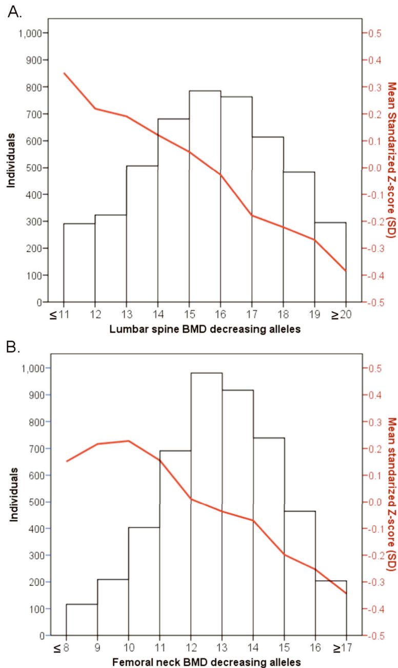
Figure 5. Histogram and line plot modeling in the Rotterdam Study the combined allelic effect across all genome-wide significant associated loci for A. Lumbar Spine BMD and B. Femoral neck BMD. Subjects were classified according to the number of BMD decreasing (risk) alleles at the lumbar spine BMD (20 SNPs) and the femoral neck (15 SNPs). The mean for each risk allele-count group was determined and the extremes of the distribution counts were pooled into the nearest risk allele-count group of size >100 individuals.
