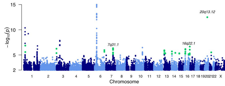
Figure 1. -\log_{10}(P) values from the 1 d.f. trend test. Alternating chromosomes shown in shades of blue. SNPs with P < 1 \times 10^{-5} which had not been previously reported are highlighted in green. The three new loci identified in this study are noted.
