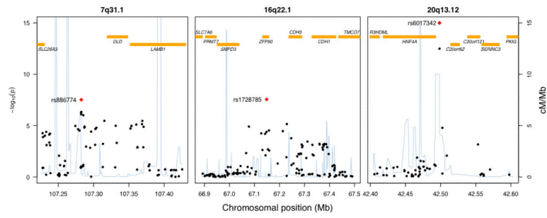
Figure 2. -\log_{10}(P) values from the 1 d.f. trend test from three new loci, along with local recombination rate estimated from HapMap data. Combined P values for replicated SNPs are indicated with a red diamond.
