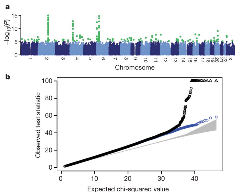
Figure 2. Genome-wide picture of geographic variation
