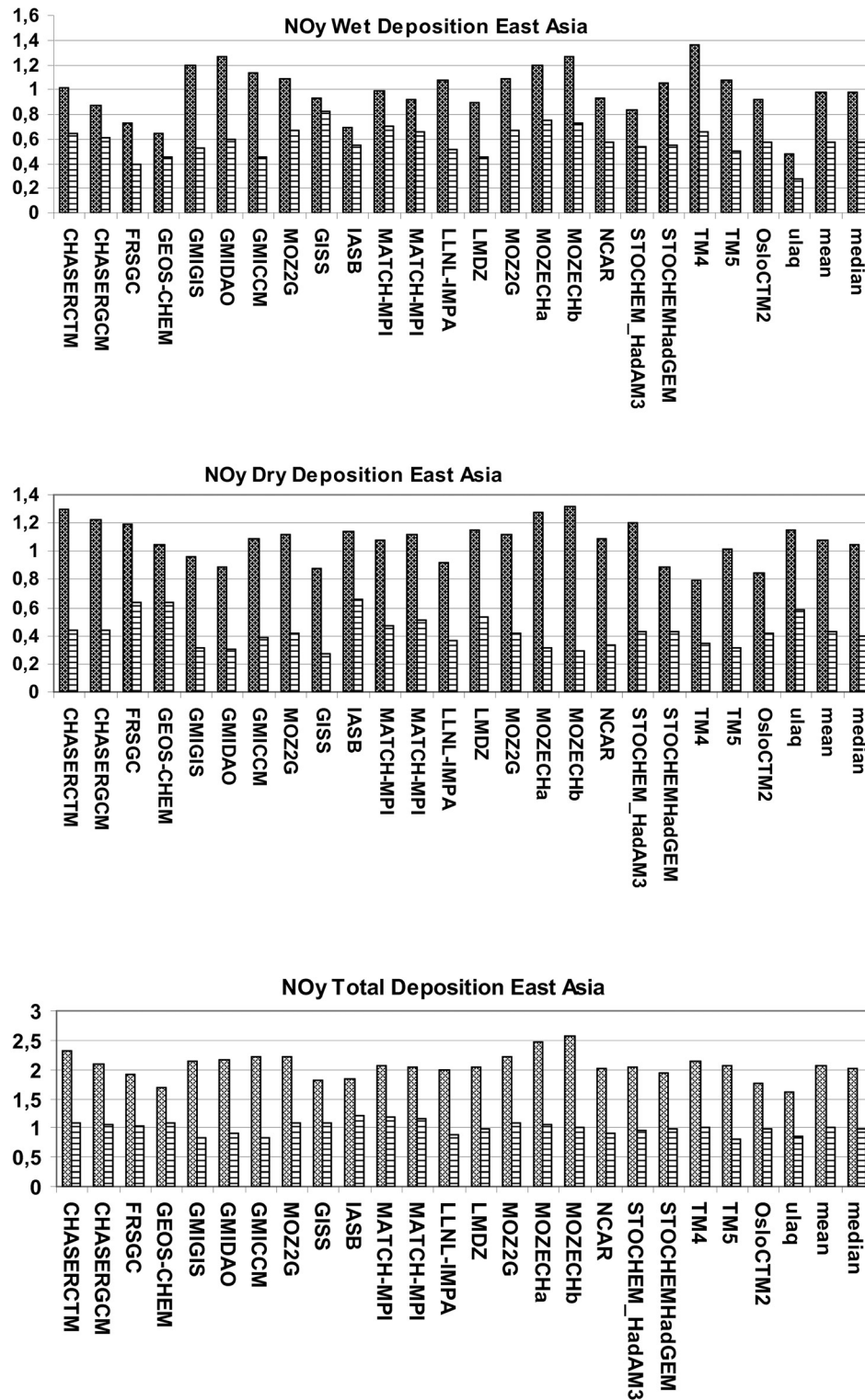
Figure 6. Analysis of the annual \text{NO}_y deposition budgets ( \text{Tg (N) yr}^{-1} ) for simulation S1 over East Asia (20°N–45°N; 110°E–130°E) analyzing the deposition over land and sea for individual models (a) \text{NO}_y wet deposition, (b) \text{NO}_y dry deposition, and (c) \text{NO}_y total deposition. Left bars denote land; right bars denote ocean.
