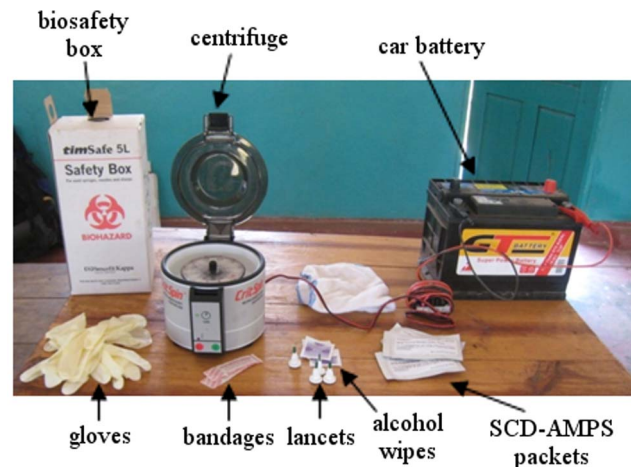
Fig. 5. Equipment for the SCD-AMPS rapid test. All the equipment necessary to run the rapid test in a rural clinic fits inside a backpack and were evaluated at rural health centers in Zambia.
