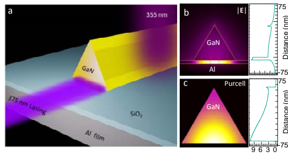
Figure 1. Ultra-violet Plasmonic Nanolaser Device. (a) Schematic of semiconductor/dielectric/plasmonic devices. GaN nanowires with a triangular cross section is supported on Al film with 8 nm SiO 2 insulator separation layer. A focused quasi-continuous wave 355 nm ultra-violet laser source is used to pump the whole GaN nanowires. The GaN photoluminescence waveguides along the high-refractive nanowire, hybridize with surface Plasmon polariton mode of Al film to produce plasmon lasing. (b) Absolute electric-field ( |E| ) distribution (left) around the plasmonic device with a wavelength of \lambda = 370 nm, corresponding to the lasing wavelength of GaN nanowires, calculated by a finite-element-method. The electric field direction is indicated by red arrows. The |E| cross section plot (right) confirms that the optical energy is confined into the insulating SiO 2 layer with a volume confinement factor of \sim \lambda^2/68 . (c) Calculated local Purcell factor distribution around the GaN nanowire (left) and cross-sectional Purcell factor plots (right). Large regime inside the nanowire exhibits a Purcell factor of \sim 7-10 .
