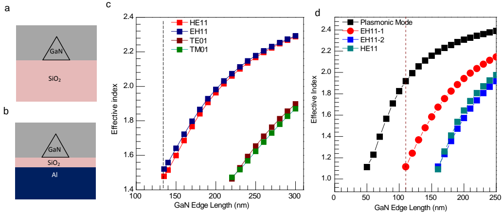
Figure 3. Modes in photonic and plasmonic devices. (a-b) Simulation configuration of photonic (a) and plasmonic devices (b). Photonic device: the GaN nanowire is sitting on a \text{SiO}_2 substrate with infinite thickness; plasmonic device: the GaN nanowire is sitting on Al substrate with a thin \text{SiO}_2 (8 nm) spacer layer. (c) The effective refractive index of HE11-like (red), EH11-like (blue), TE01-like (wine) and TM01-like (Oliver) mode versus the GaN nanowire edge length a . The cut-off sizes of HE11-like and EH11-like mode are around a = 135 nm (dashed line). (d) The effective indexes of hybrid plasmon mode (black), photonic EH11-1-like (red), EH11-2-like (green), HE-11-like (blue) modes versus the GaN nanowire edge length in plasmonic device. The cut-off size of EH11-1-like mode is around a = 110 nm (dashed line).
