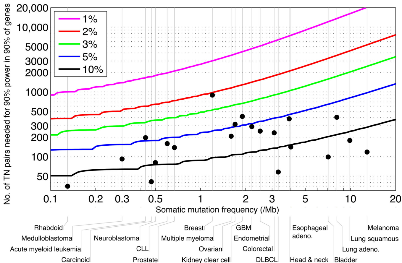
Figure 5. Number of samples needed to detect significantly mutated genes, as a function of a tumor type’s median background mutation frequency of (x-axis) and a cancer gene’s mutation rate above background (the various curves). Y-axis shows the number of samples needed to achieve 90% power for 90% of genes. Grey vertical lines indicate tumor type median background mutation frequencies. Black dots indicate sample sizes in the current study. For most tumor types, the current sample size is inadequate to reliably detect genes mutated at 5% or less above background. See also Supplementary Figure 9.
