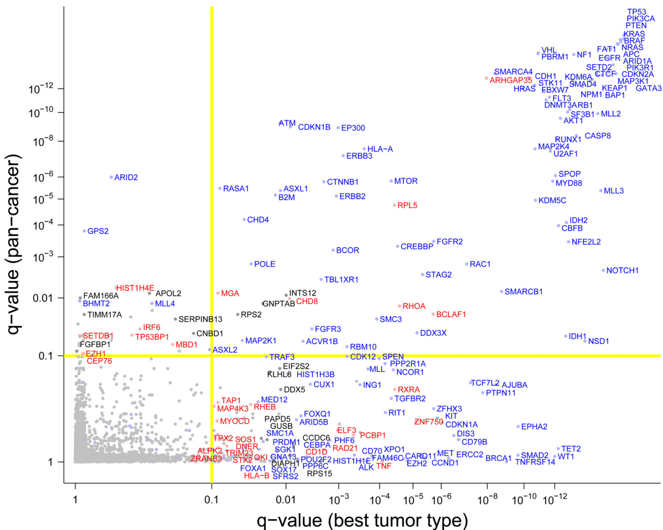
Figure 3. Cancer genes identified in 4742-tumor dataset. X-axis indicates the q-value (FDR) in the most significant of the 21 tumor types. Y-axis indicates the q-value when the 4742 tumors are analyzed as a combined cohort. Genes in the upper left quadrant reached significance only in the combined analysis. Genes in the lower right quadrant reached significance only in one or more single-type analyses. Genes in the upper right quadrant were significant in both the combined set and in individual tumor types. Color of gene names is as in Figure 2.
