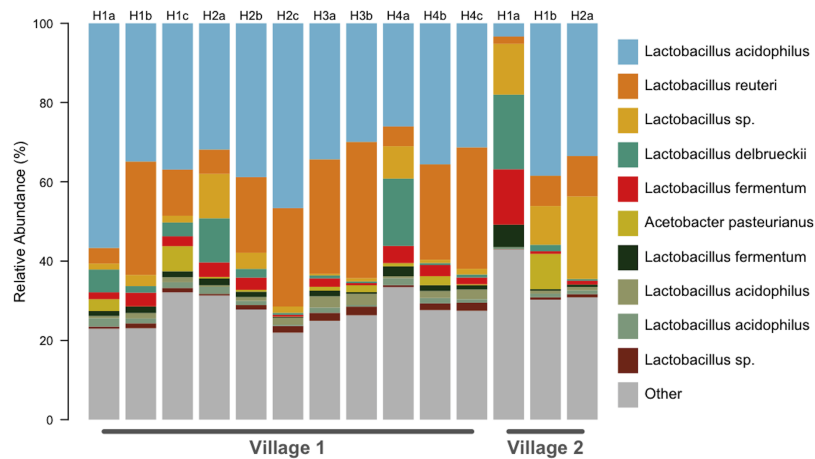
Figure 1 All chicha samples were dominated by Lactobacillus spp. OTU predicted identities are from a manual BLAST search against the NCBI 16S isolate database. We found ten OTUs with greater than 1% relative abundance. This barplot shows the relative abundance (%) of ten most common bacteria isolates for each sample. Up to three independent batches were sampled for each house (e.g., H1a–H1c). Eleven samples were analyzed from Village 1 and three from Village 2.
