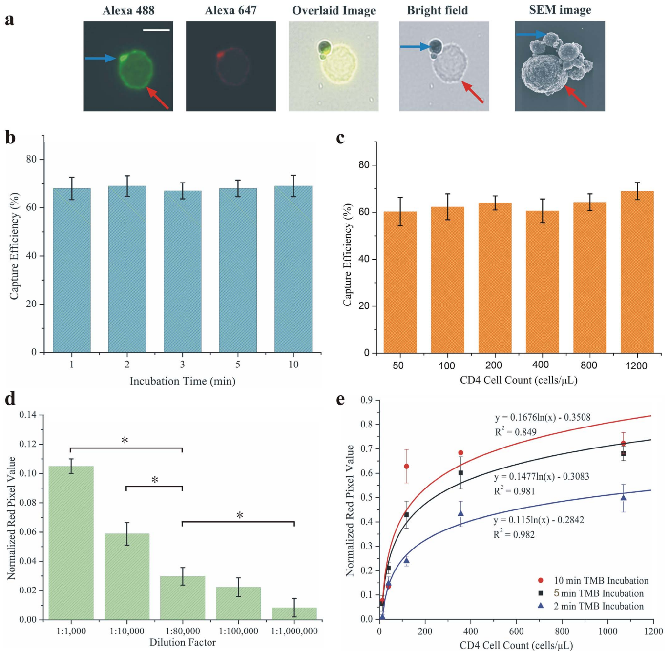
Figure 2 | Characterization of m-ELISA for CD4 cell count. (a) Capture of CD4 + T lymphocytes (red arrow) on magnetic beads (blue arrow). Magnetic beads were incubated with whole blood and the captured T lymphocyte was stained with anti-CD4 Alexa Fluor 488 and anti-CD3 Alexa Fluor 647. The fluorescent images of Fluor 488, Alexa Fluor 647, bright-field, as well as the overlaid image (by ImageJ software) demonstrate capture of CD4 + T lymphocytes by magnetic beads. The scanning electron microscope (SEM) image validates the capture of CD4 + T lymphocyte on magnetic beads. The scale bar is 10 \mu m. (b) Efficiency of magnetic beads for capturing CD4 + T lymphocytes at varying incubation times. 25 \mu L of functionalized magnetic beads (10 mg/mL) were incubated with whole blood containing 1,000 cells/ \mu L CD4 + T lymphocyte. The unbound T lymphocytes in the supernatant were quantified by flow cytometry, which was used to calculate the capture efficiency. One-way ANOVA was performed to analyze and no statistical significance ( p > 0.05 ) was found. (c) Efficiency of magnetic beads for capturing CD4 + T lymphocytes at varying concentrations of CD4 + T lymphocytes. The same procedure as mentioned in (b) was used to calculate the capture efficiency. One-way ANOVA analysis indicated that there was no significant difference in capture efficiency ( p > 0.05 ). (d) Optimization of HRP-antibody in m-ELISA. The variable, HRP-conjugated antibody was diluted at different concentrations and tested with plasma samples, which served as negative control. 1 : 80,000 was chosen for the following experiments since this concentration was the highest concentration of HRP-antibody that avoided false positive results. A mobile application was used to extract red (R) pixel values from the color development region on-chip and normalized them according to the background as shown in the Y-axis. One-way ANOVA was performed to analyze the color intensity caused by excessive HRP ( n = 3 , * indicates the statistical significance, p < 0.05 ). (e) Whole blood from a healthy blood sample was serially diluted (undiluted, 1 : 3, 1 : 9, 1 : 27 and 1 : 81) used to construct the standard curve with different 3, 3', 5, 5' Tetramethylbenzidine (TMB) incubation periods. Each data point was performed in triplicates and the standard deviation was shown.
