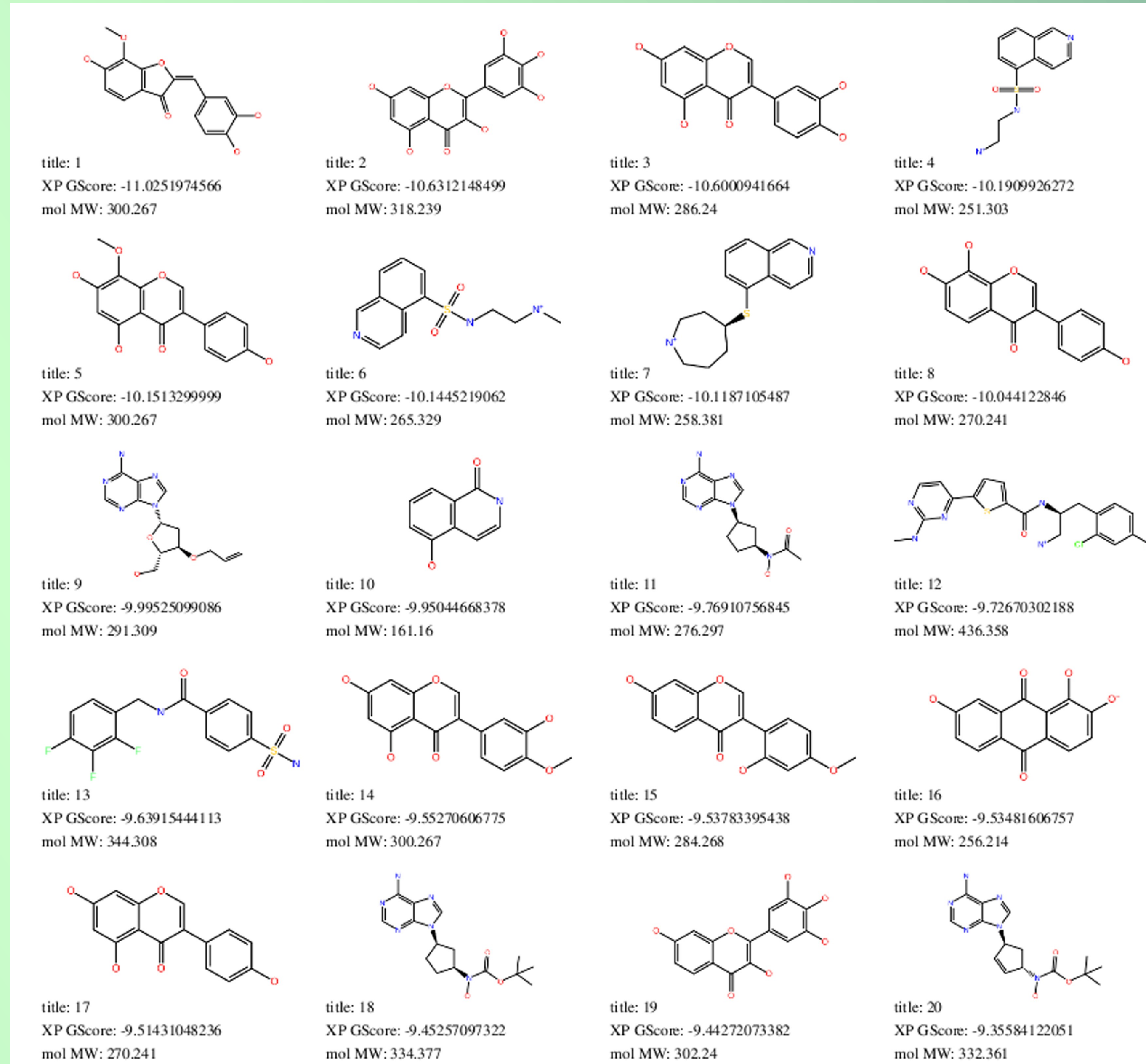
Figure 5. Predicted 20 best lead molecules based on the XP Gscore
